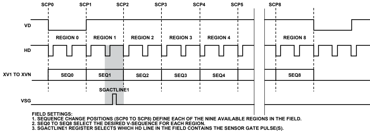
Figure 49. Complete Field is Divided into Regions
