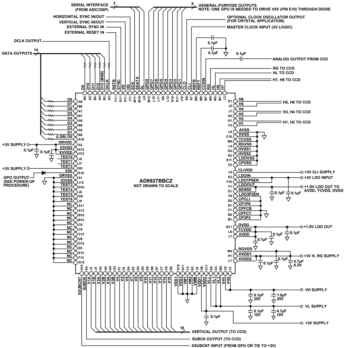
Figure 94. Typical 3 V Circuit Configuration
