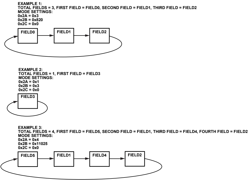
Figure 67. Using the MODE Registers to Select Field Timing
