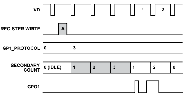
Figure 75. ShotDelay Toggle Operation Using GP_PROTOCOL = 3
