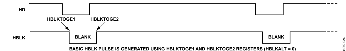
Figure 25. Typical Horizontal Blanking Pulse Placement (HBLKMODE = 0)
