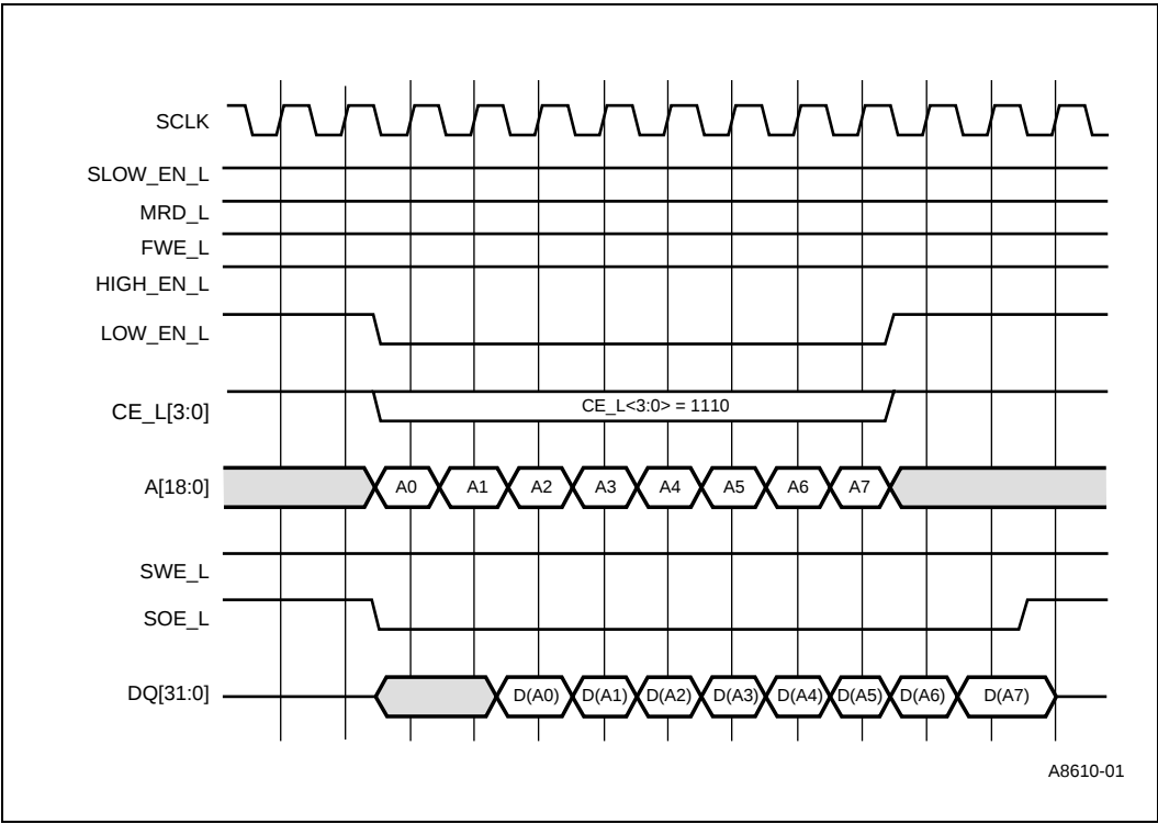
Figure 63. Pipelined SRAM Read Burst of Eight Longwords
