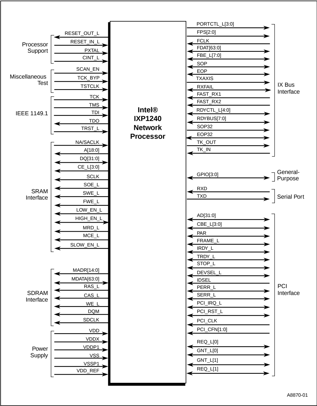
Figure 6. Pinout Diagram
