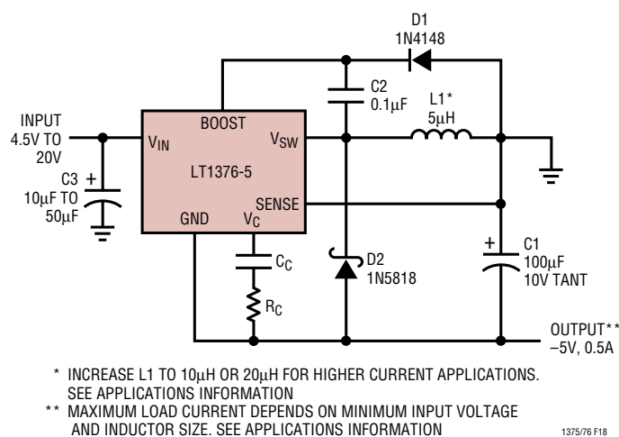
Figure 18. Positive-to-Negative Converter
