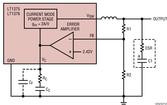
Figure 12. Model for Loop Response
