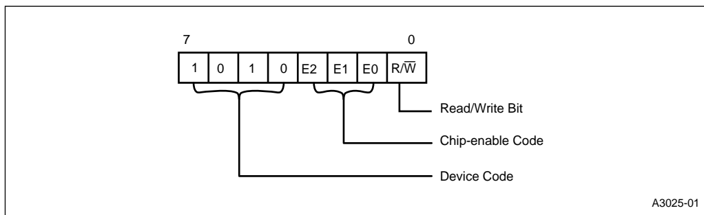
Figure 3. Device-select Byte
