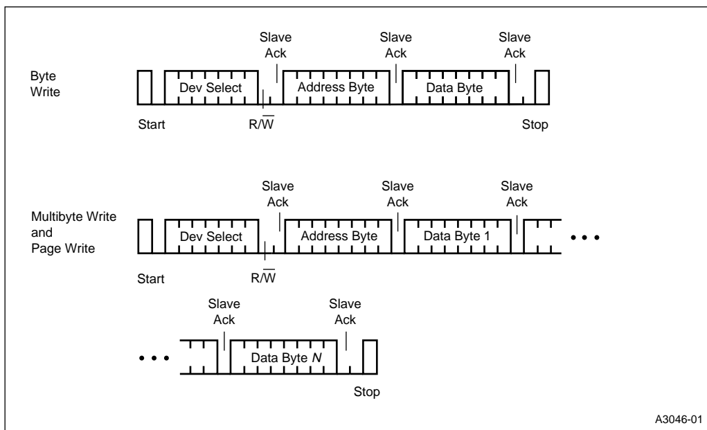
Figure 4. Write Operations
