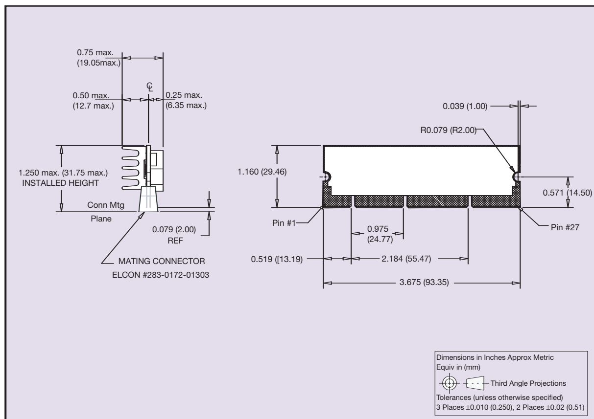
Figure 5: Mechanical Drawing
