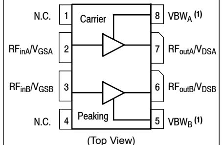
Figure 1. Pin Connections
