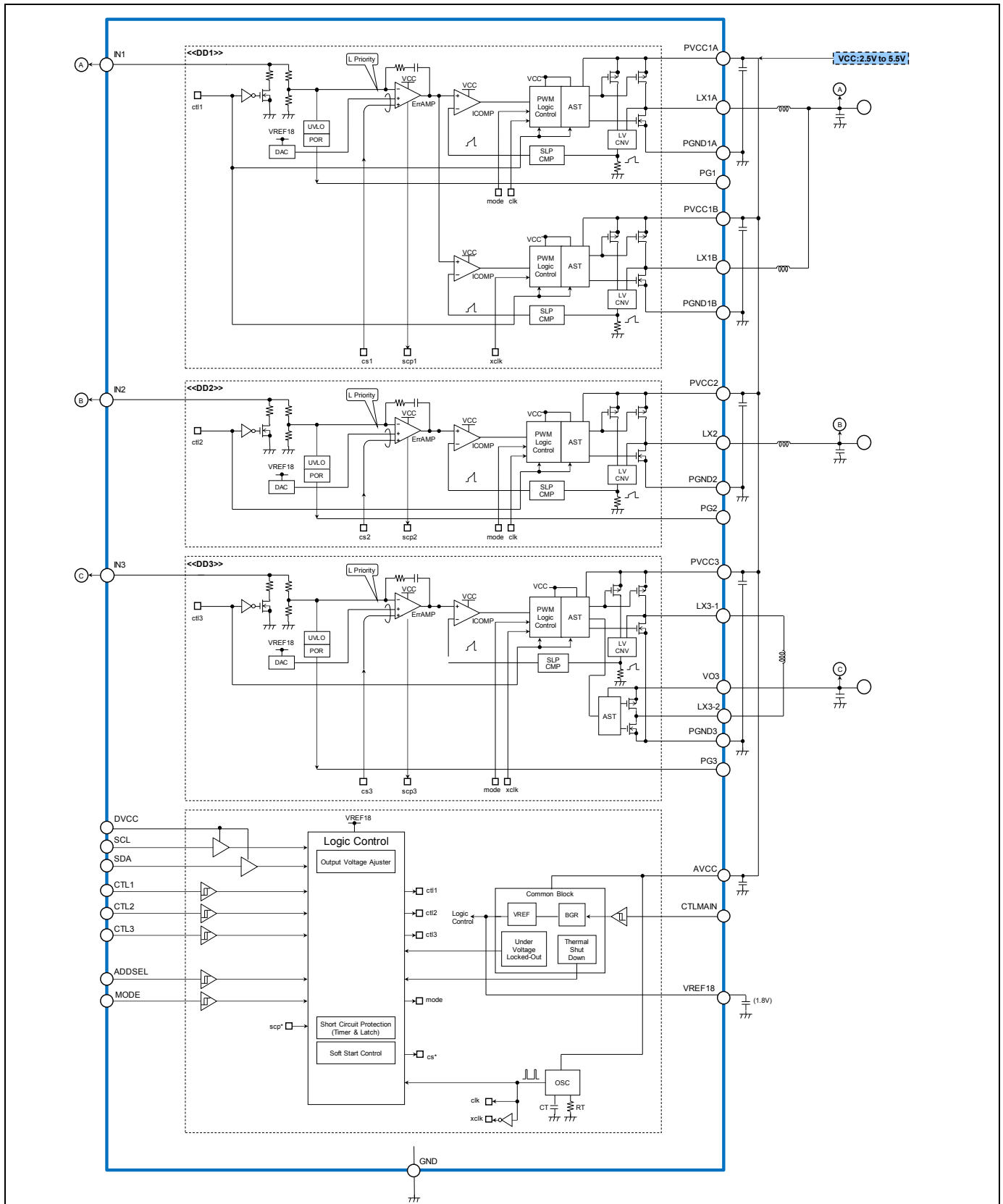
Figure 8-1 Block Diagram
