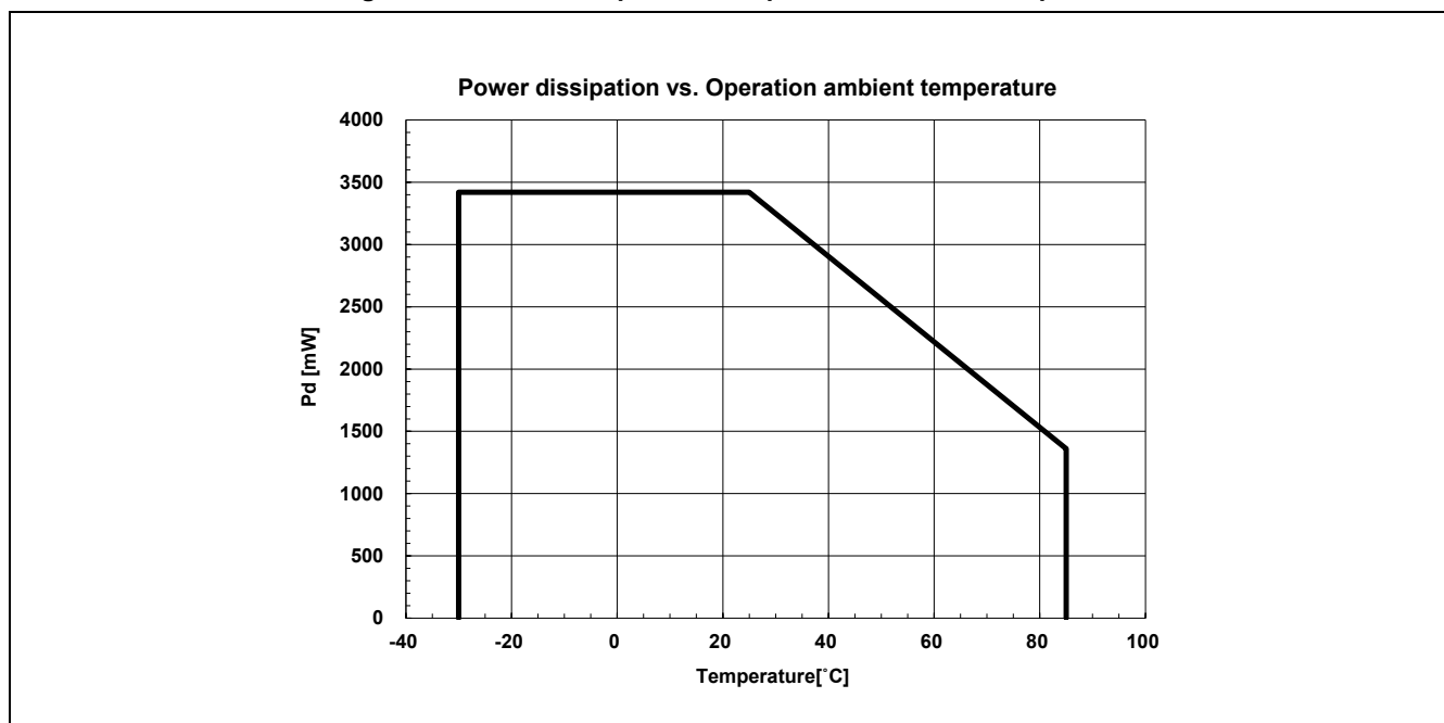
Figure 9-1 Power Dissipation vs. Operation Ambient Temperature
