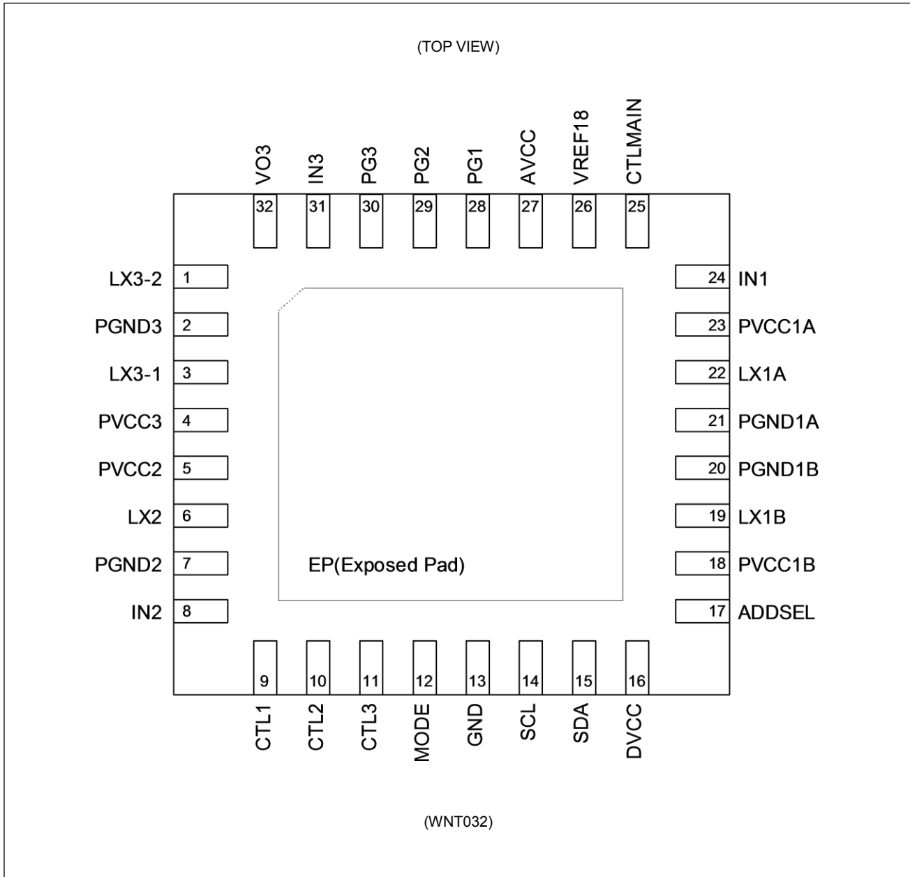
Figure 6-1 Pin Configuration
