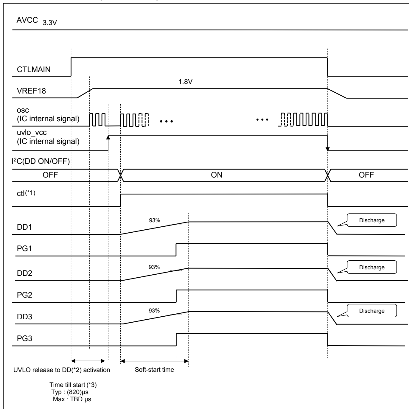
Figure 16-1 Turning on and off Sequence (AVCC → CTLMAIN → I 2 C)
