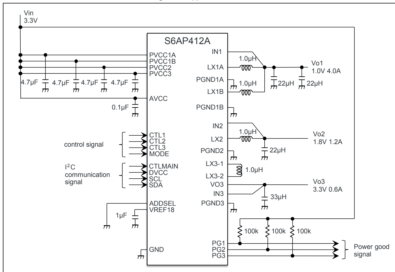
Figure 4-1 Application Circuit
