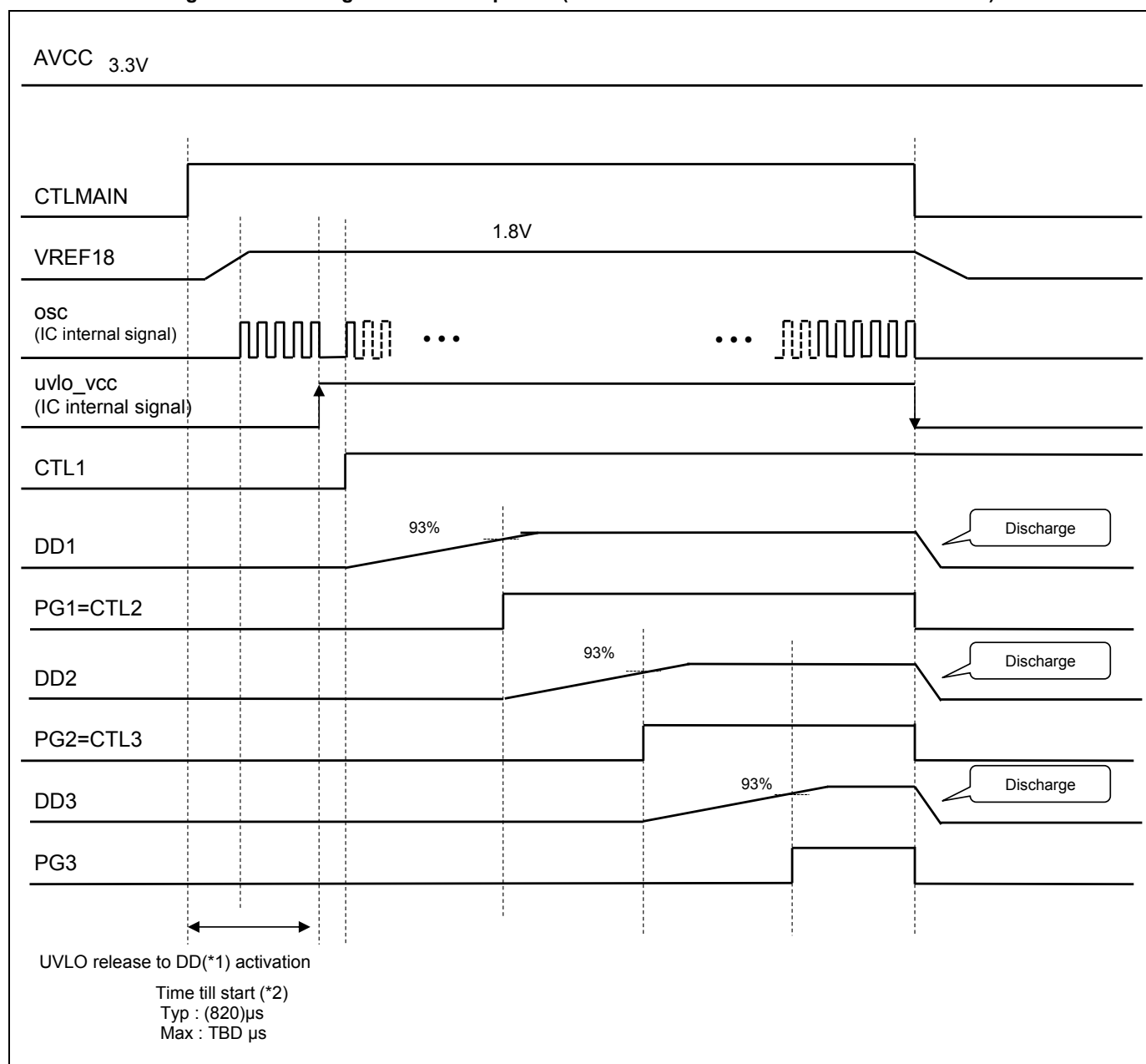
Figure 15-1 Turning on and off Sequence (AVCC → CTLMAIN → CTL1 → CTL2 → CTL3)
