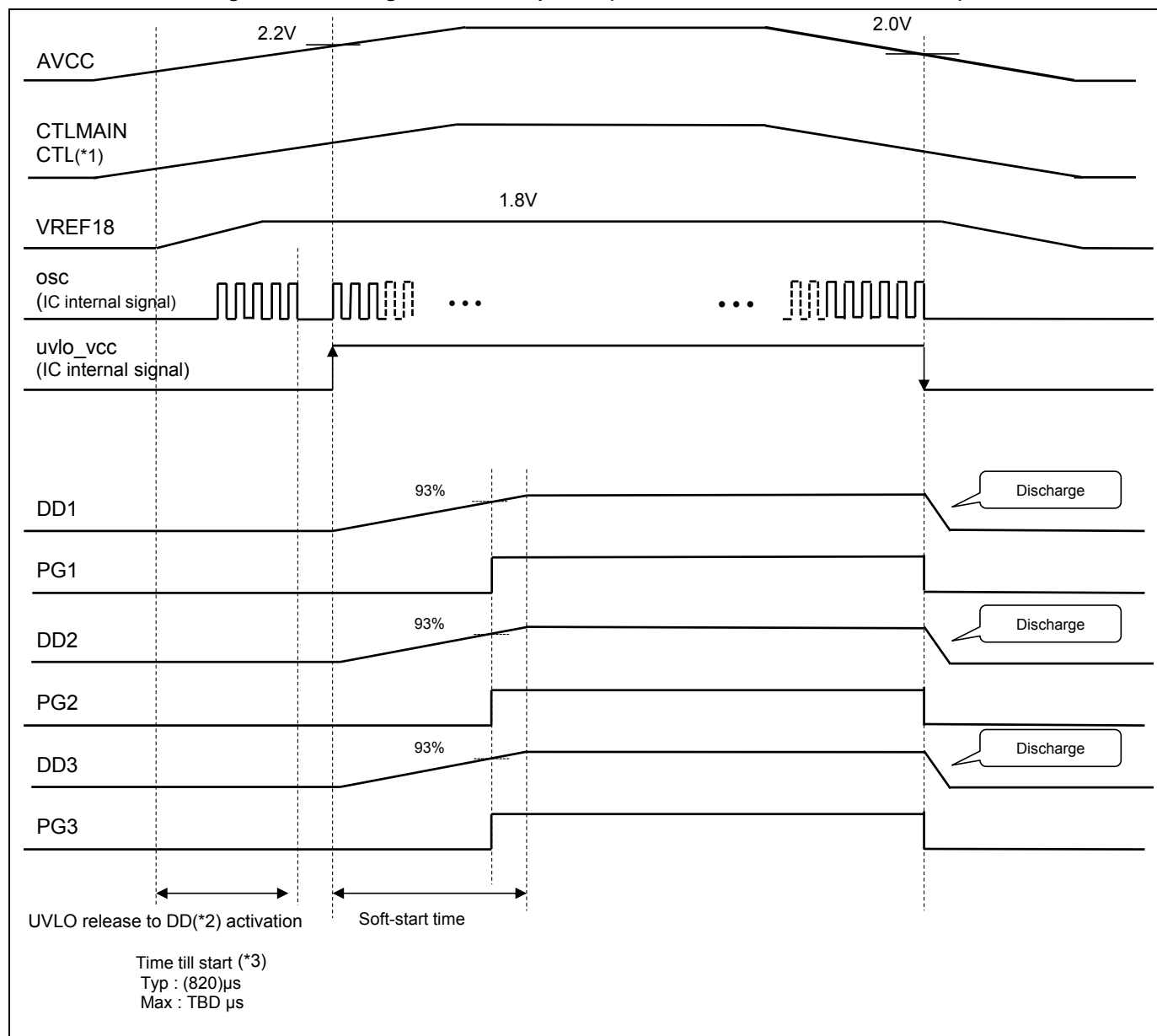
Figure 14-1 Turning on and off Sequence (AVCC=CTLMAIN, CTL1, CTL2, CTL3)
