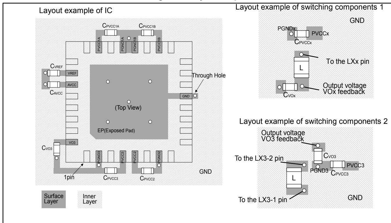
Figure 31-1 Layout example
