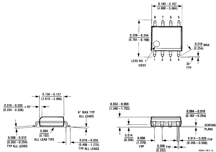
SO Package (M) Order Number DS8921M, DS8921AM or DS8921ATM NS Package Number M08A
