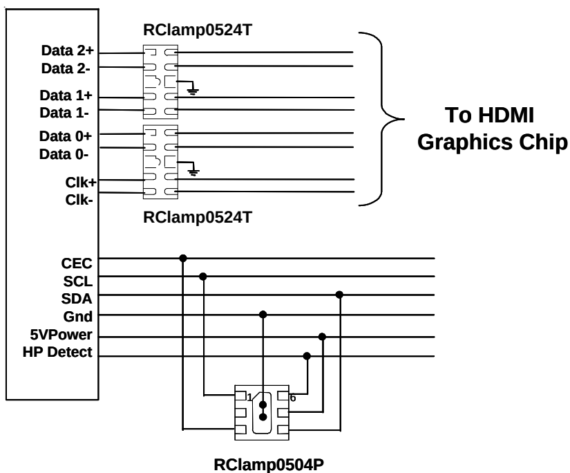
Figure 4. HDMI Protection
