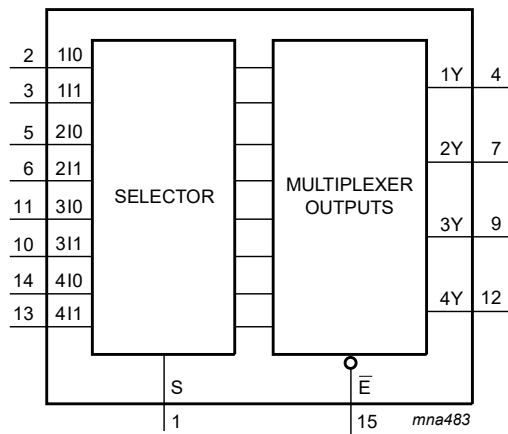
Fig. 3. Functional diagram
