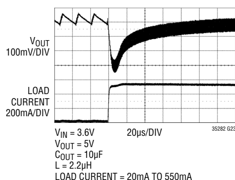
Load Step Response (Burst Mode Operation, 3.6V to 5V)
