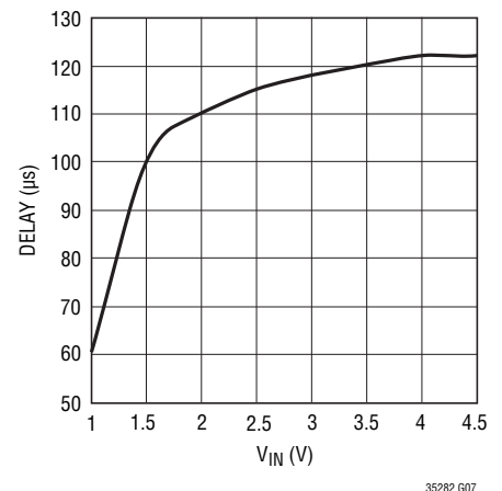
Start-Up Delay Time vs V_{IN}
