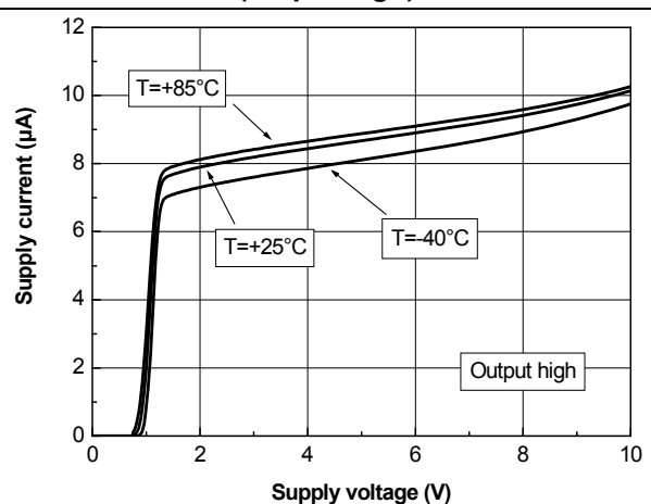
Figure 2. Supply current vs. supply voltage (output high)
