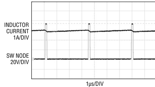
96% MAXIMUM DUTY CYCLE WITH D_{MAX} = \text{SGND}
