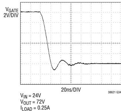
Gate Turn-Off Waveform Driving Renesas HAT2267H
