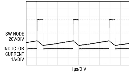
84% MAXIMUM DUTY CYCLE WITH D_{MAX} = \text{FLOAT}
