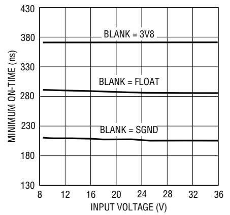
Minimum On-Time vs Input Voltage
