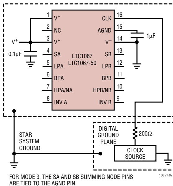
Figure 2. Single Supply Ground Plane Connections
