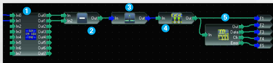
1. Virtual Probe 2. Difference 3. Interpolate 4. Tapped Delay Line Filter 5. Equalized Receiver
