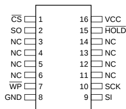
16-pin SOIC
