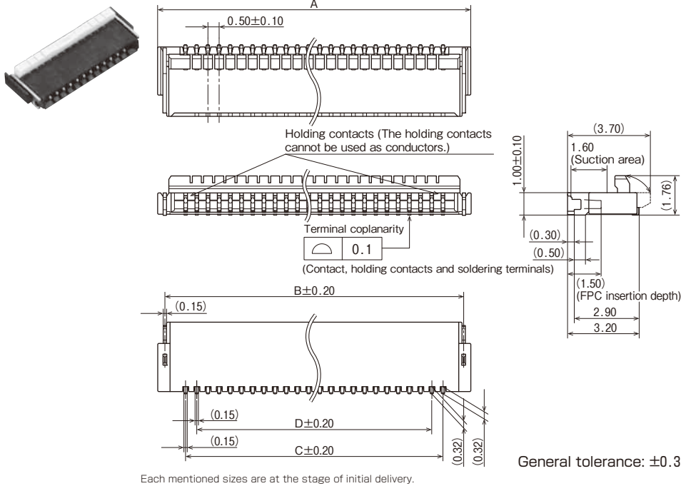
Dimension table
