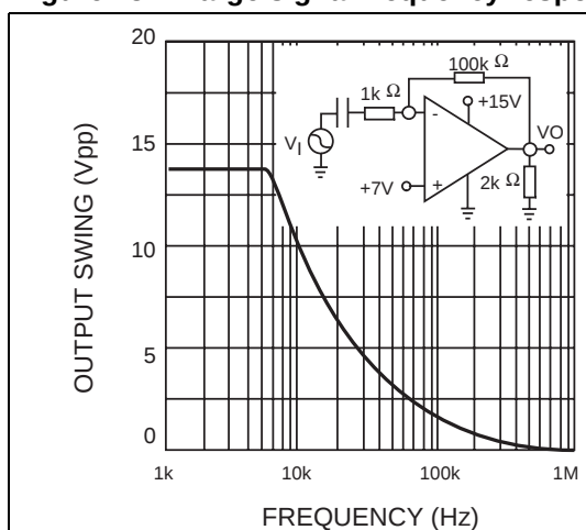
Figure 13. Large signal frequency response
