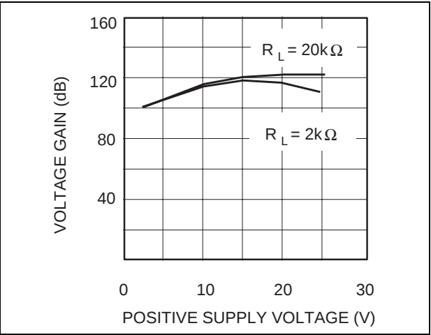
Figure 16. Voltage gain
