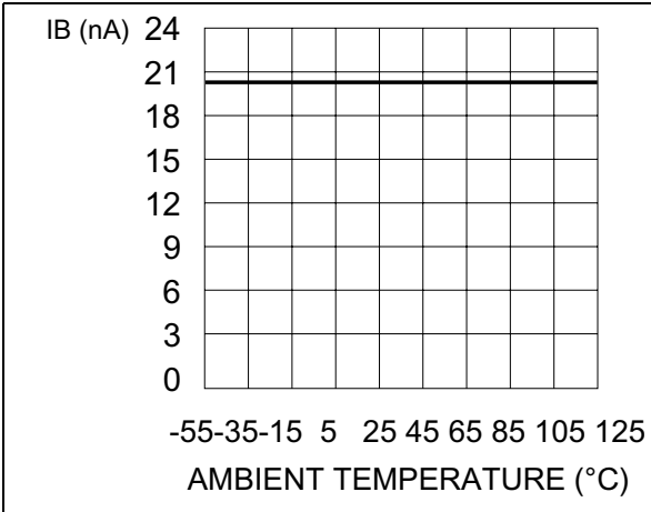
Figure 3. Input bias current vs. T_{amb}
