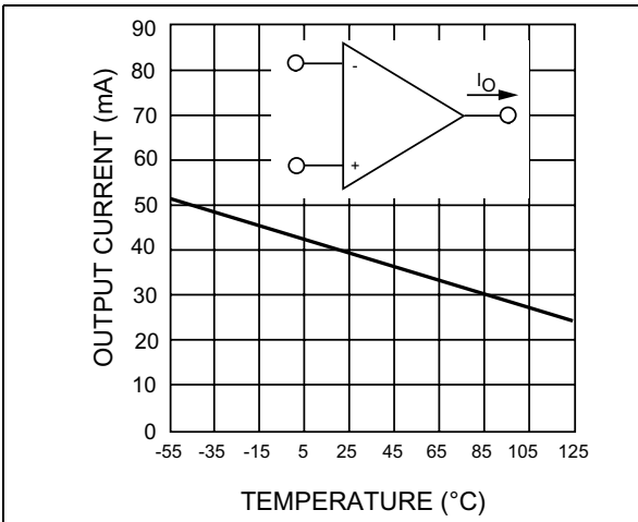
Figure 5. Current limiting
