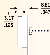
Window Mount Side View
