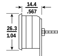
Backlit Bezel Mount Side View
