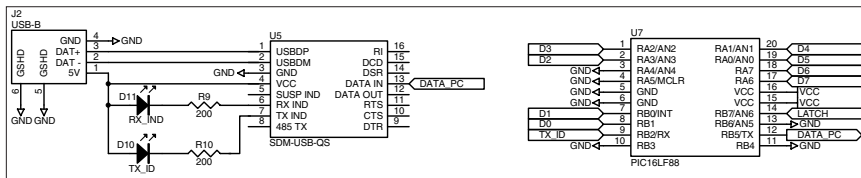
Figure 14: USB Section
