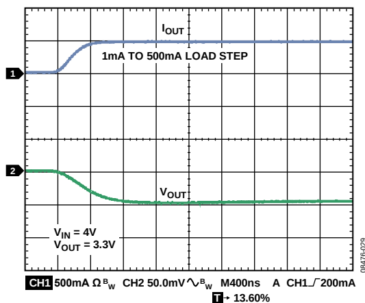
Figure 31. Output Transient Response, C_{OUT} = 4.7 \mu\text{F}
