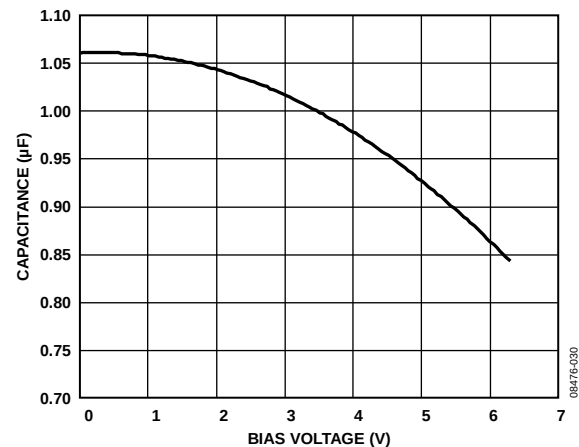
Figure 32. Capacitance vs. Capacitor Voltage Bias Characteristics
