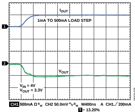
Figure 30. Output Transient Response, C_{OUT} = 1 \mu\text{F}
