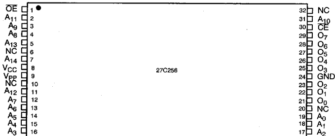
32-Pin TSOP Top View
