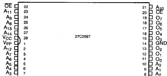
28-Pin TSOP Top View
