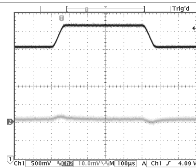
Figure 16. Load Transient (LDO2)
