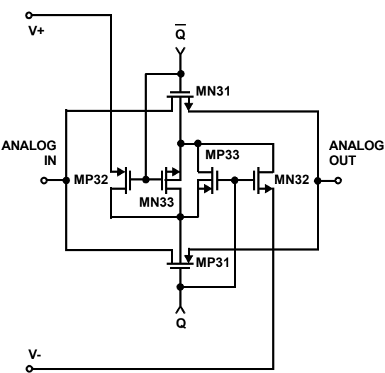
SWITCH CELL
