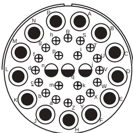
40-64 - 3 20 13 12 16 8 (Coax) RG-124/U
