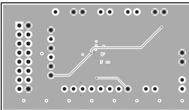
Figure 3. Middle Layer 2
