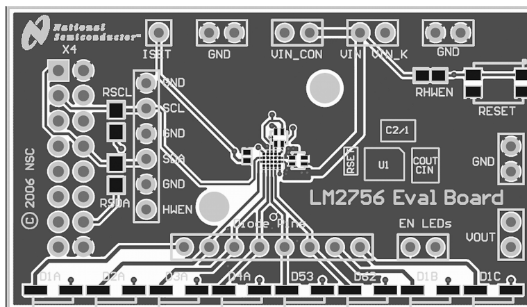
Figure 1. Top Layer
