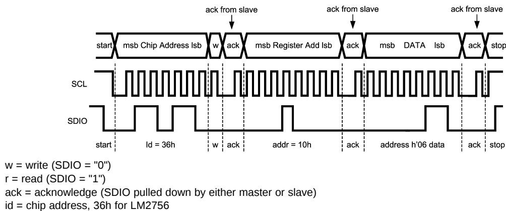
Figure 7. Write Cycle
