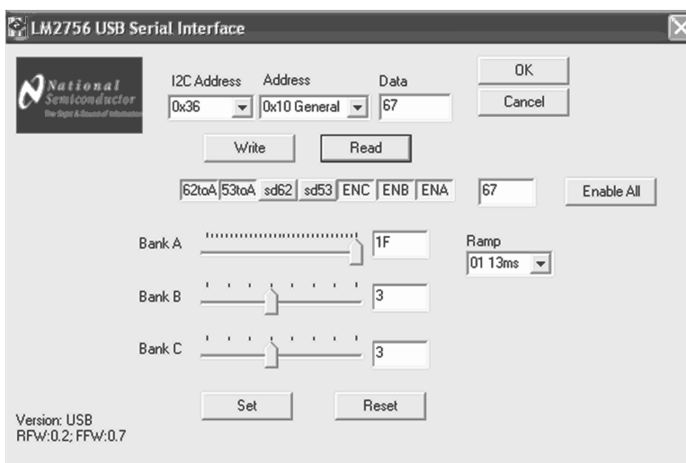
Figure 20. Example Configuration
