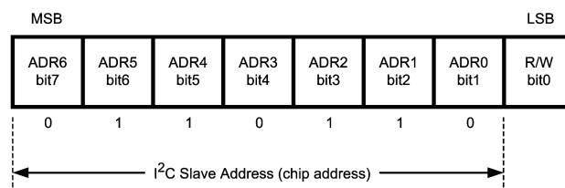
Figure 8. Chip Address
