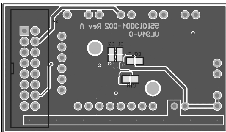
Figure 4. Bottom Layer (unmirrored)
