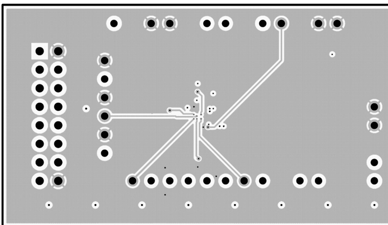
Figure 2. Middle Layer 1
