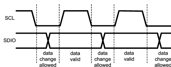
Figure 5. Data Validity Diagram
