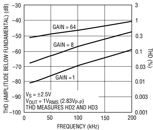
LTC6910-2 Distortion with Heavy Loading ( R_L = 500\Omega )
