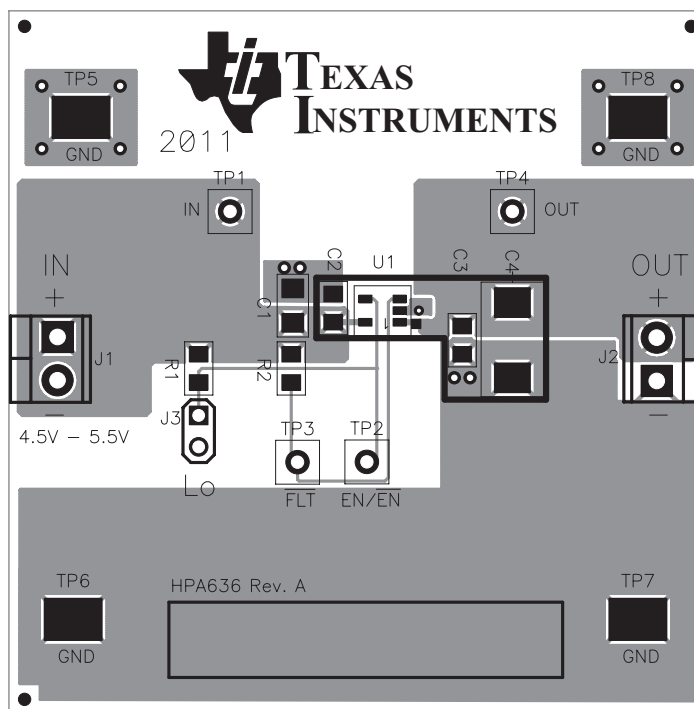
Figure 3. TPS20xxCDBVEVM-636 Component Placement
