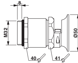
Dimensioned drawing
