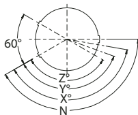
Keyway Positions, Shell Size 7-12
