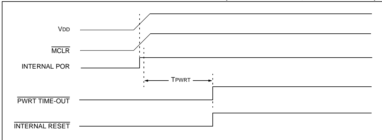
FIGURE 4-3: TIME-OUT SEQUENCE ON POWER-UP ( \overline{\text{MCLR}} TIED TO \text{V}_{\text{DD}} , \text{V}_{\text{DD}} RISE < \text{TPWRT} )
