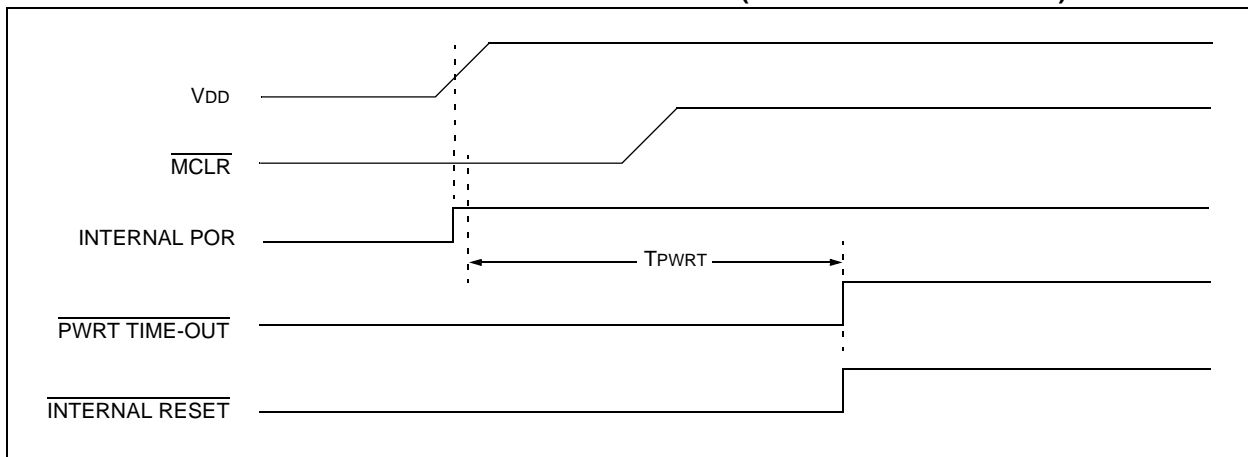
FIGURE 4-4: TIME-OUT SEQUENCE ON POWER-UP ( \overline{\text{MCLR}} NOT TIED TO \text{V}_{\text{DD}} ): CASE 1
