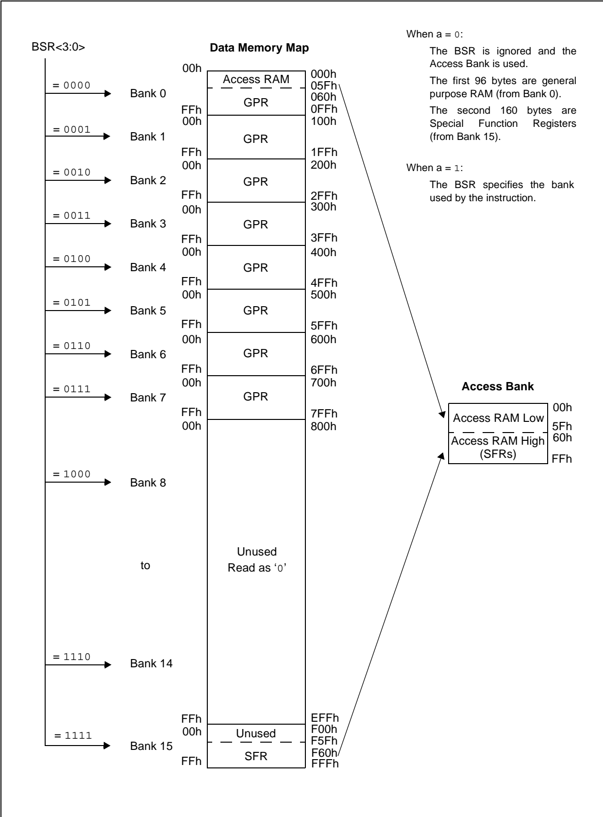
FIGURE 5-7: DATA MEMORY MAP FOR PIC18FX5J10/X5J15/X6J10 DEVICES
