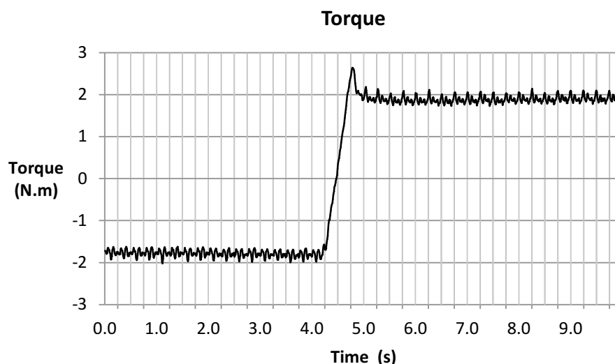
Figure 14-24. Torque Plot
