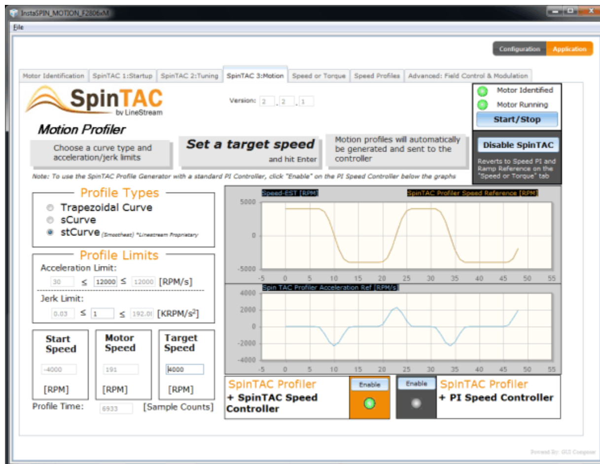
Figure 2-5. InstaSPIN-MOTION™ GUI Using SpinTAC 3:Motion Tab
