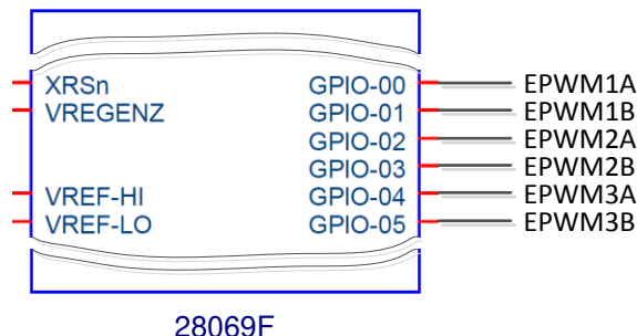
Figure 5-13. PWM Pin Configuration
