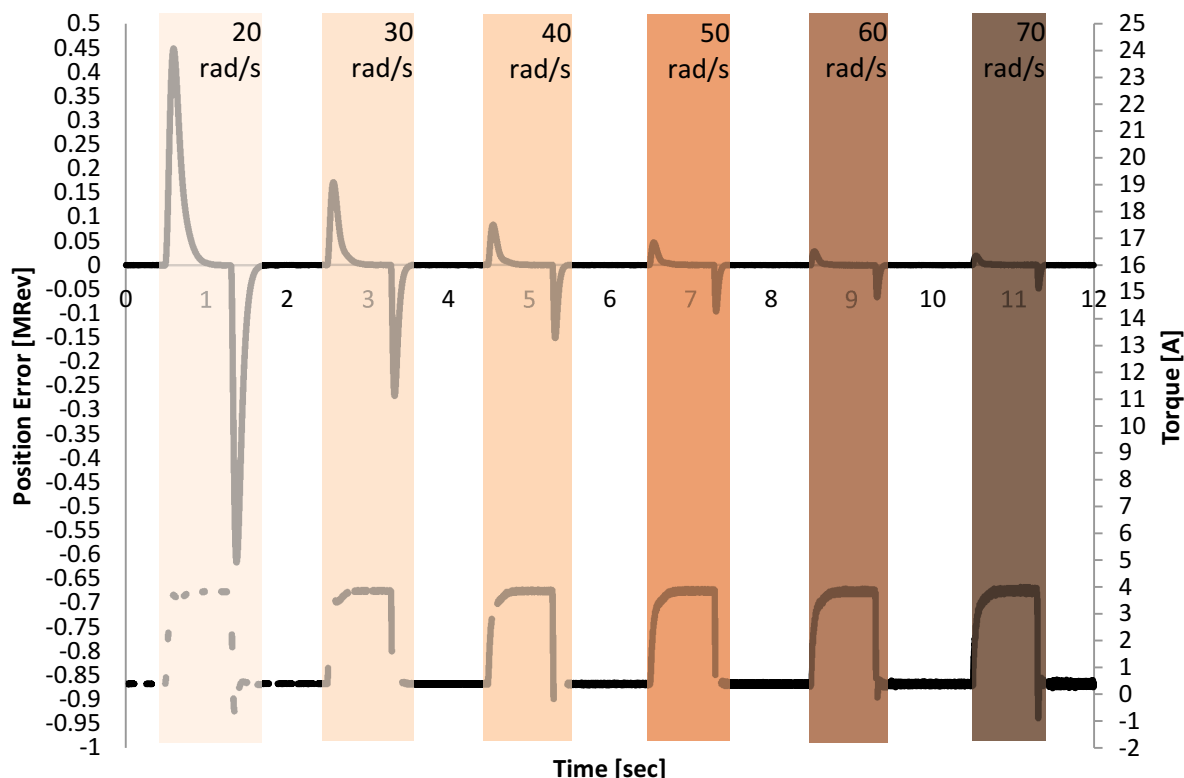
Figure 12-7. Comparison of Bandwidths for SpinTAC™ Position Control
