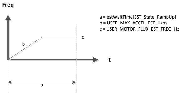
Figure 6-17. Ramp-Up Timing
