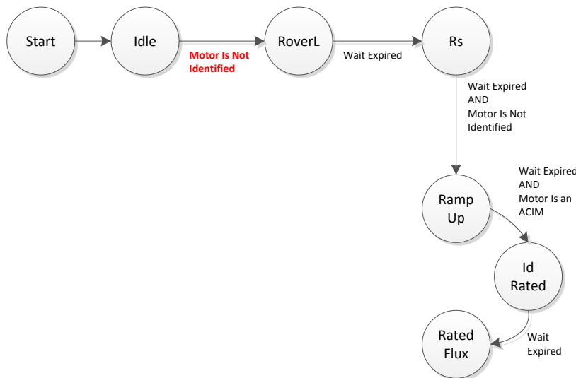
Figure 6-34. ACIM Rated Flux EST State
