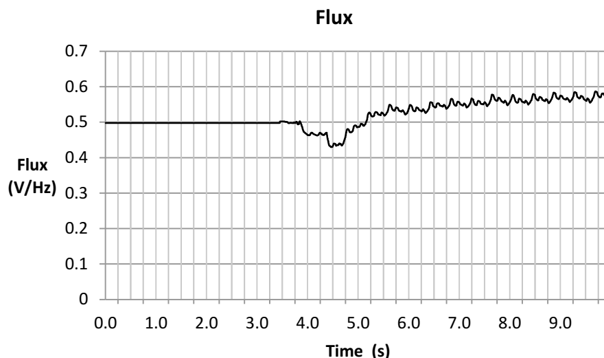
Figure 14-43. Flux Plot
