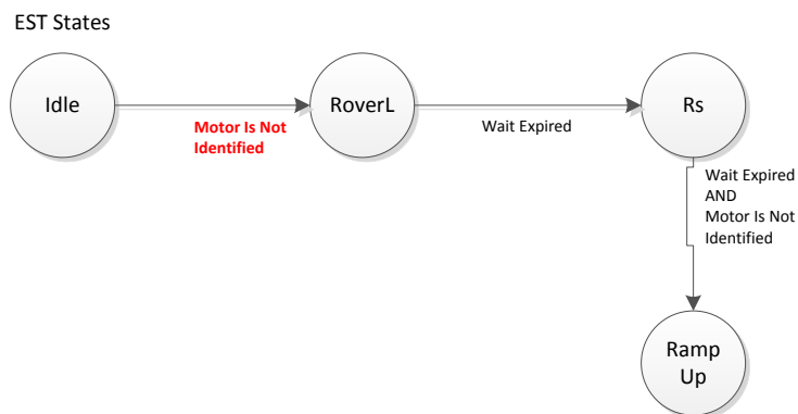
Figure 6-16. Ramp-Up EST State
