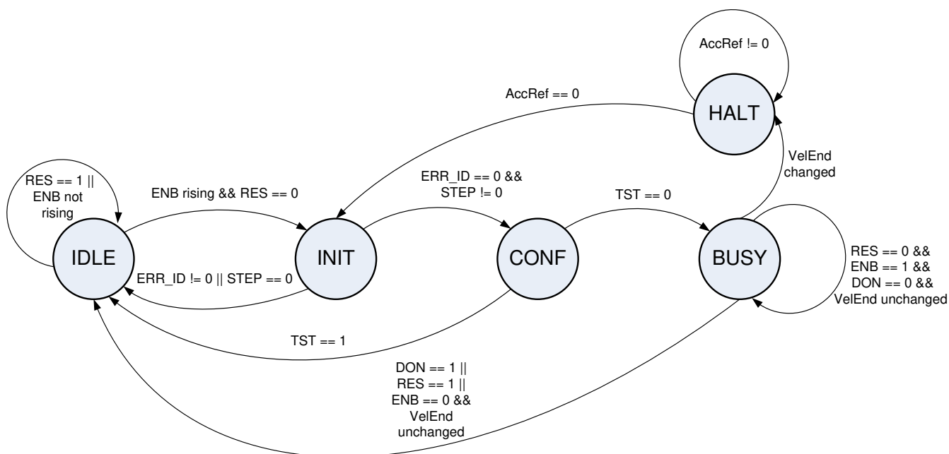
Figure 3-8. SpinTAC™ Velocity Move State Transition Map
