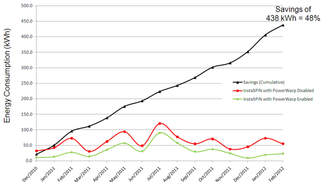
Figure 16-8. InstaSPIN-FOC™ with PowerWarp™ Software Enabled vs. InstaSPIN-FOC™ with PowerWarp™ Software Disabled
