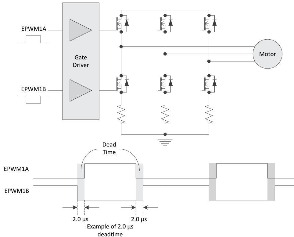
Figure 5-11. Dead-Time Configuration
