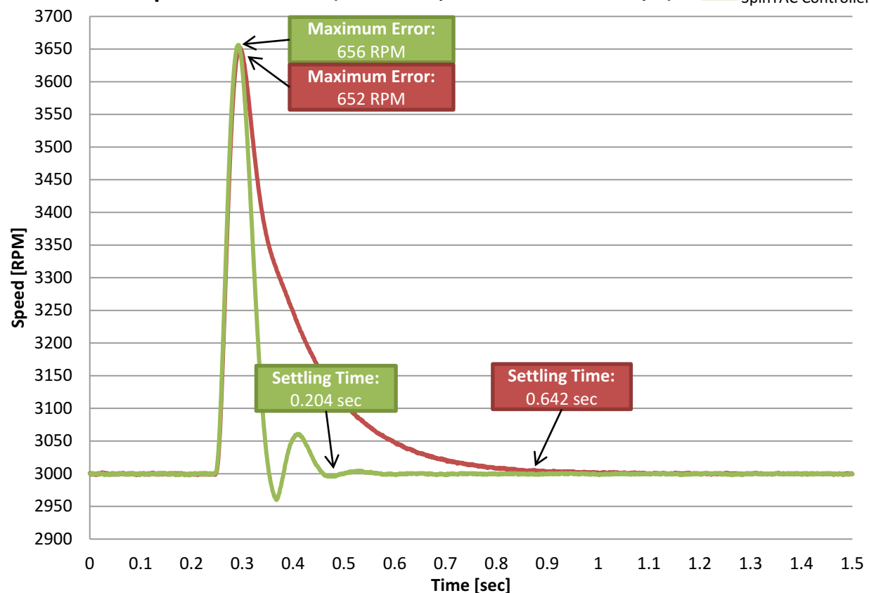
Figure 12-12. PI and SpinTAC™ Comparison for Removed Torque Disturbance Velocity Control
