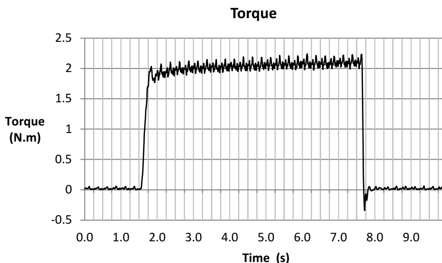
Figure 14-9. Torque Plot
