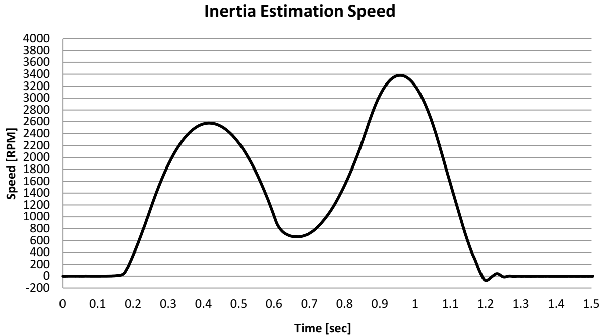
Figure 7-6. SpinTAC™ Velocity Identify Speed Feedback
