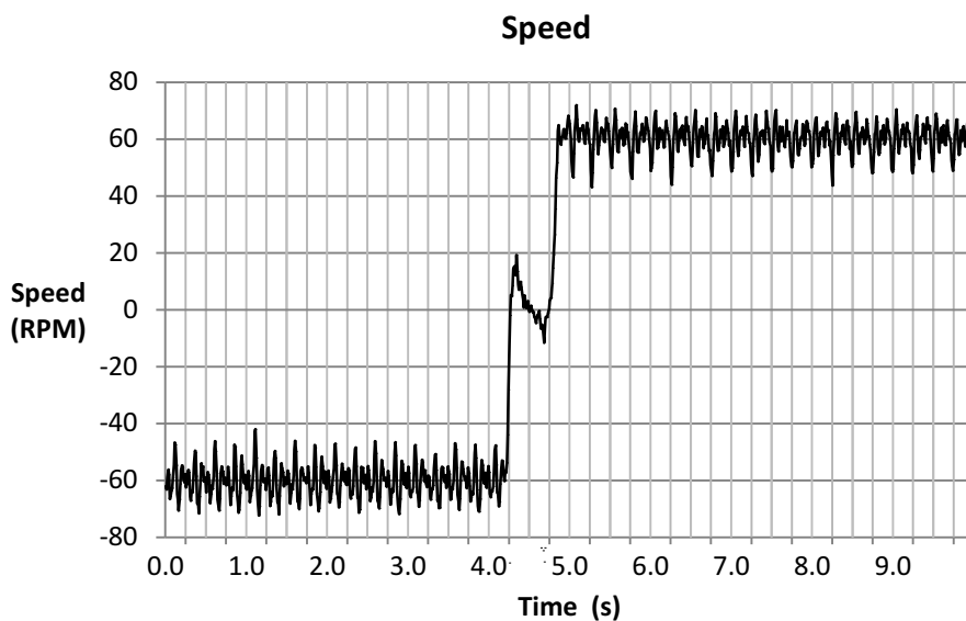
Figure 14-23. Speed Plot
