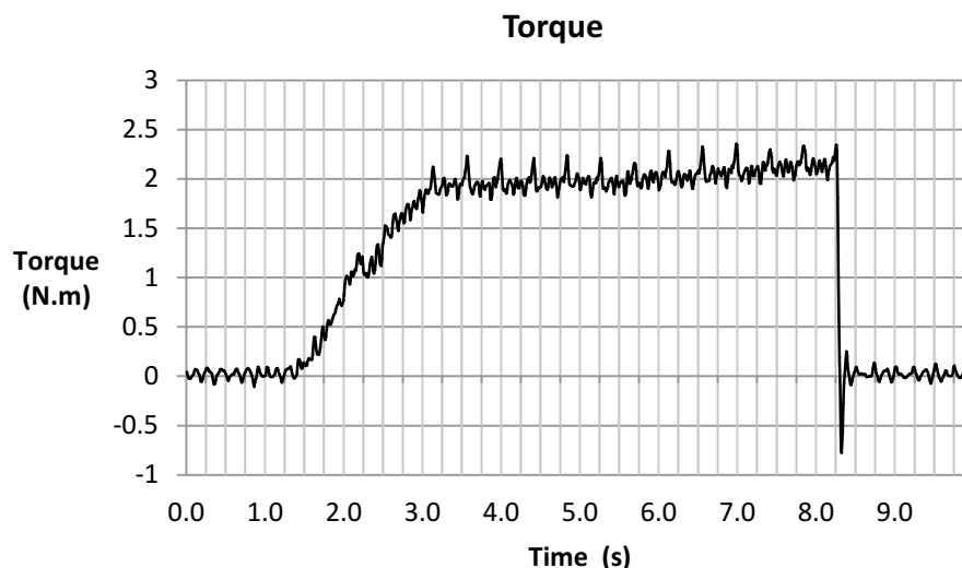
Figure 14-17. Torque Plot
