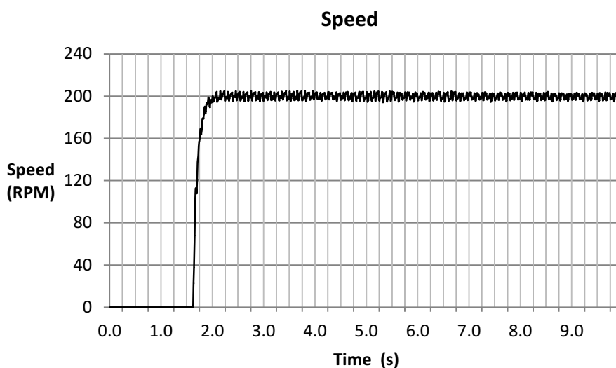
Figure 14-61. Speed Plot
