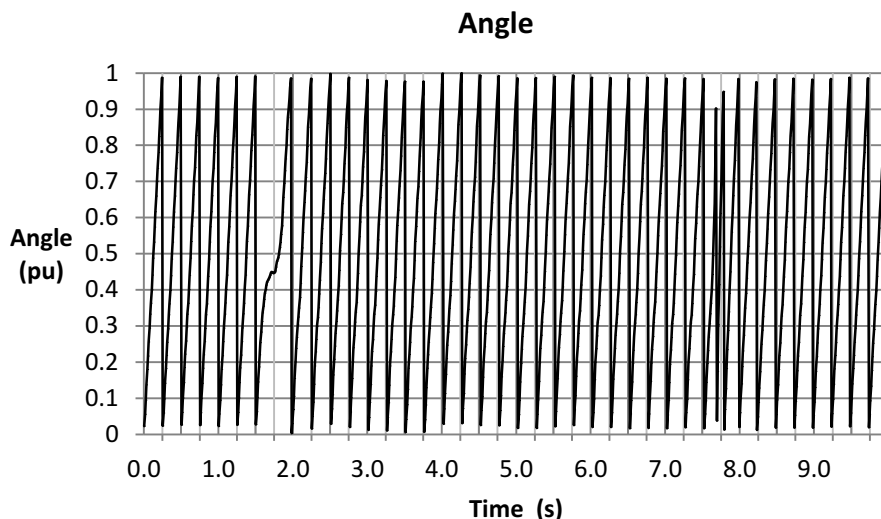
Figure 14-5. Angle Plot
