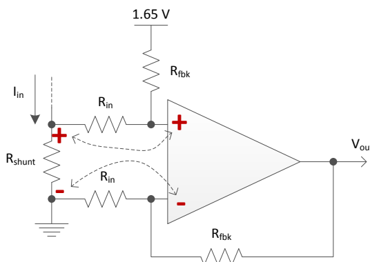
Figure 5-5. Positive Feedback
