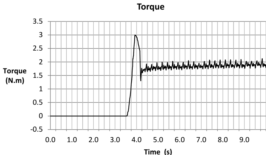
Figure 14-40. Torque Plot
