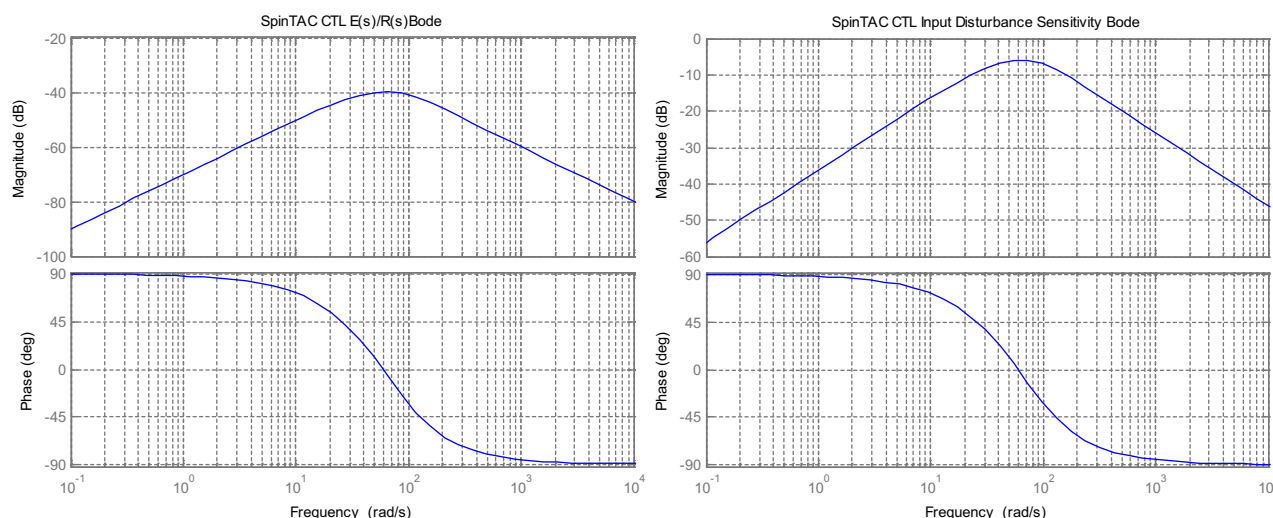
Figure 12-4. Typical Performance Bode of SpinTAC™ Velocity Control
