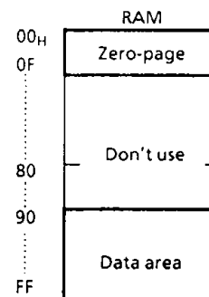
Figure 2. RAM addressing
