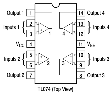
N SUFFIX PLASTIC PACKAGE CASE 646 (TL074 Only)
