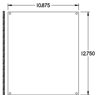
INNER PANEL
