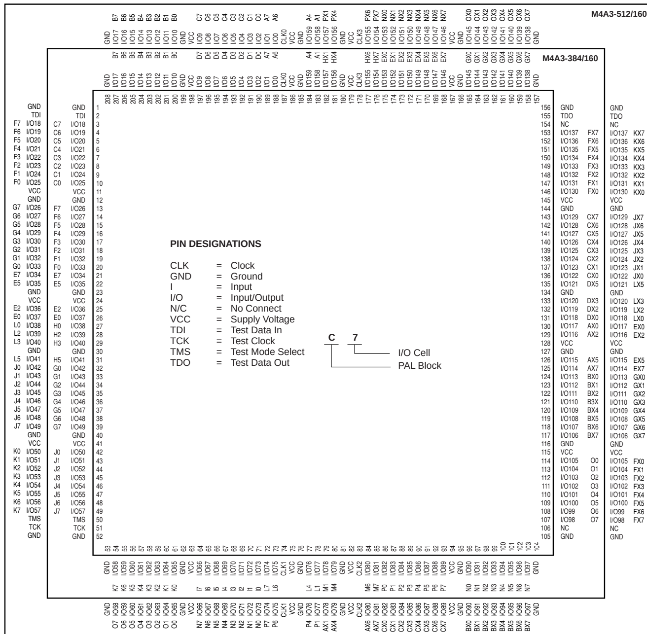
208-Pin PQFP
