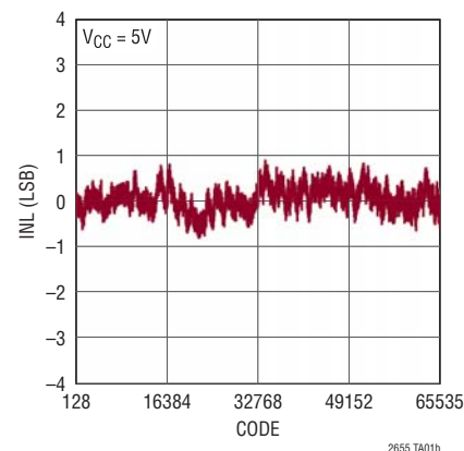
INL Curve
