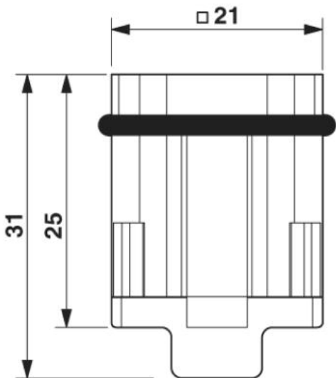
Dimensioned drawing
