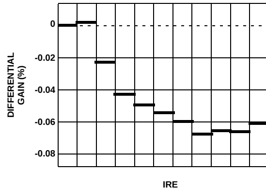
FIGURE 16. DIFFERENTIAL GAIN
