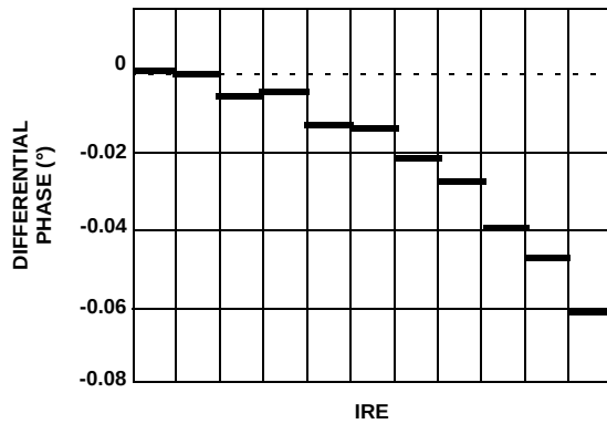
FIGURE 17. DIFFERENTIAL PHASE
