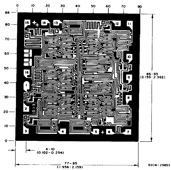
Dimensions and pad layout for CD4018B.
