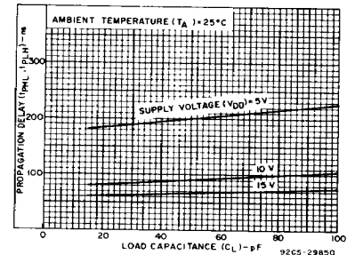
Fig. 8 - Typical propagation delay time as a function of load capacitance (CLOCK to Q).
