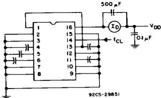
Fig. 14 — Dynamic power dissipation test circuit.
