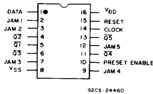
TERMINAL DIAGRAM Top View
