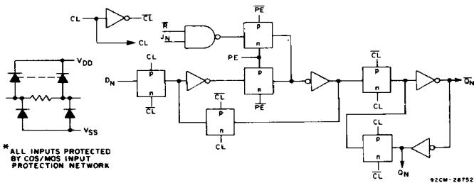
Fig. 2 — Detail of a typical stage.
