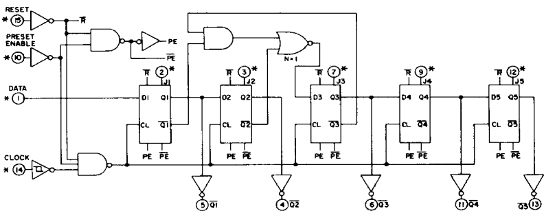
Fig. 1 — Logic diagram.
