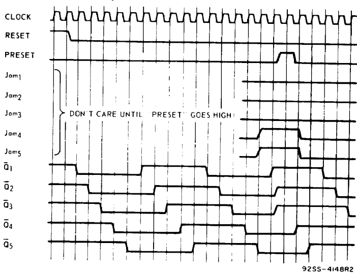
Fig. 15 — Timing diagram.
