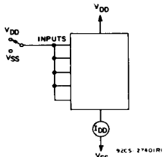
Fig. 11 — Quiescent device current test circuit.
