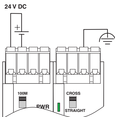
Figure 2 Connecting the supply voltage
