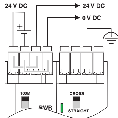
Figure 3 Voltage continuation
