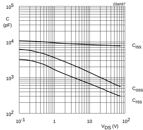
Fig 11. Input, output and reverse transfer capacitances as a function of drain-source voltage; typical values.
