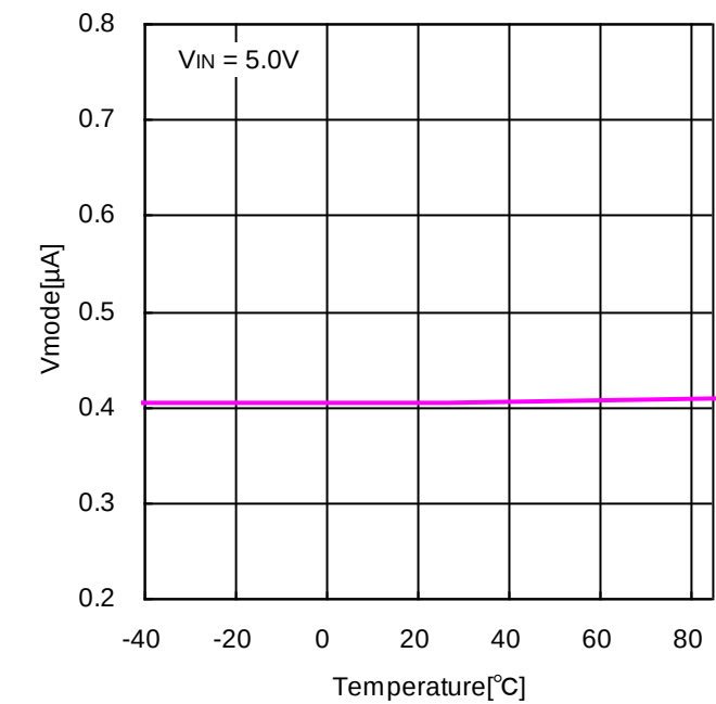
Figure 10. Mode Threshold vs Temperature
