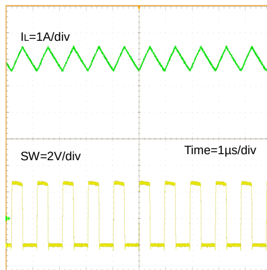
Figure 35. Switching Waveform ( V_{IN}=5.0V , V_{OUT}=1.8V , I_{OUT}=6A , L=1.5\mu H )
