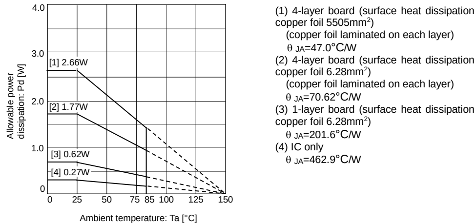
Figure 56. Thermal Derating Characteristics (VQFN016V3030)
