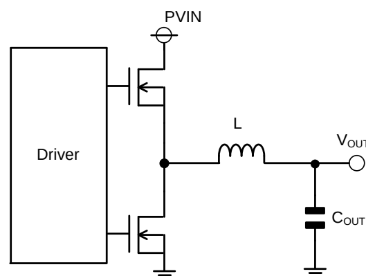
Figure 50. Output LC Filter Circuit
