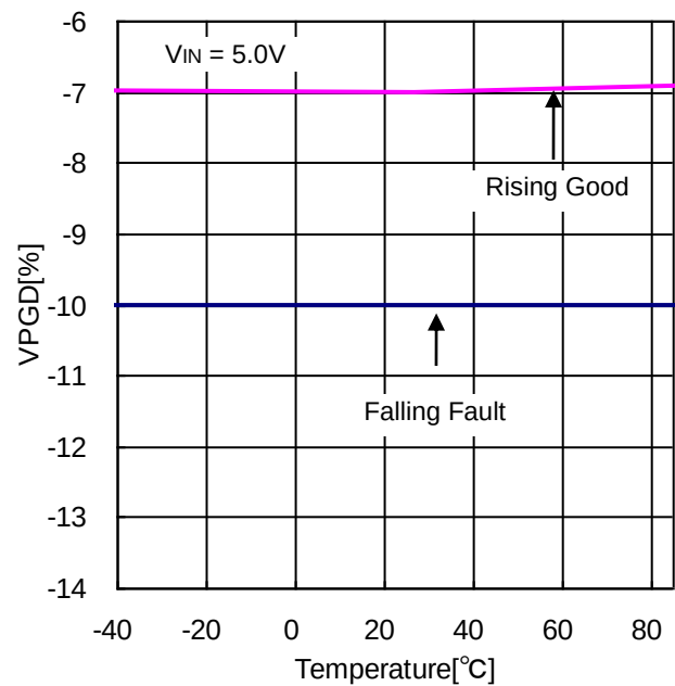
Figure 16. PGD Falling Voltage vs Temperature
