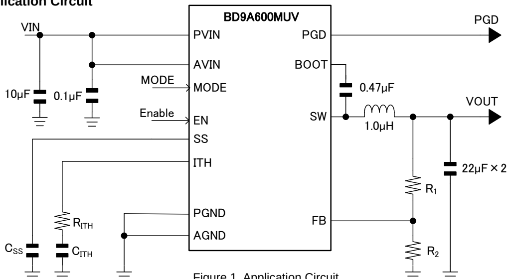
Figure 1. Application Circuit
