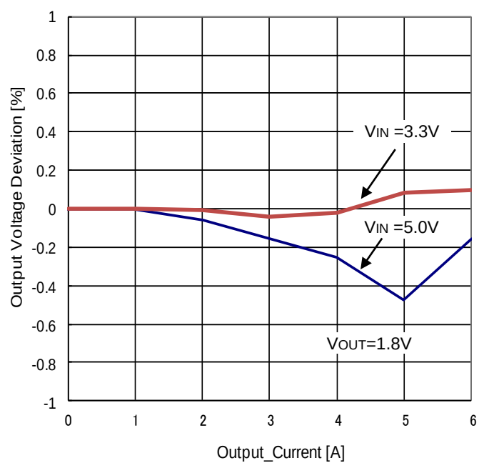
Figure 38. Load Regulation vs Load Current
