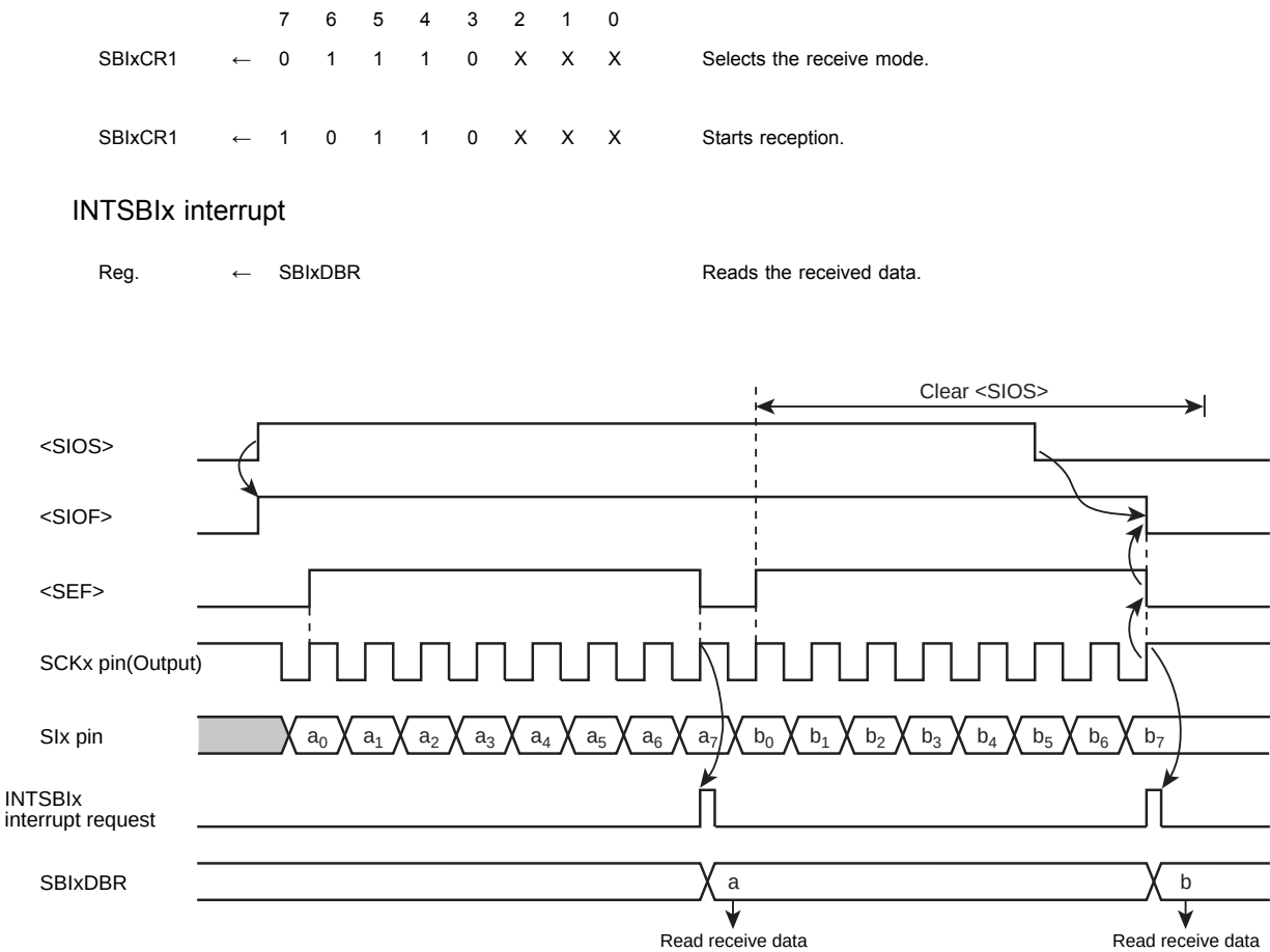
Figure 14-19 Receive Mode (Example: Internal Clock)
