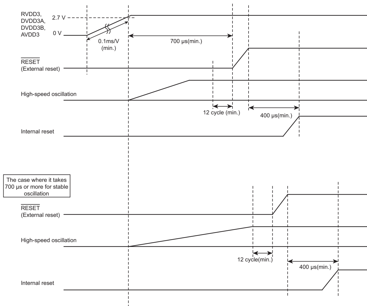
Figure 5-1 Cold Reset Sequence
