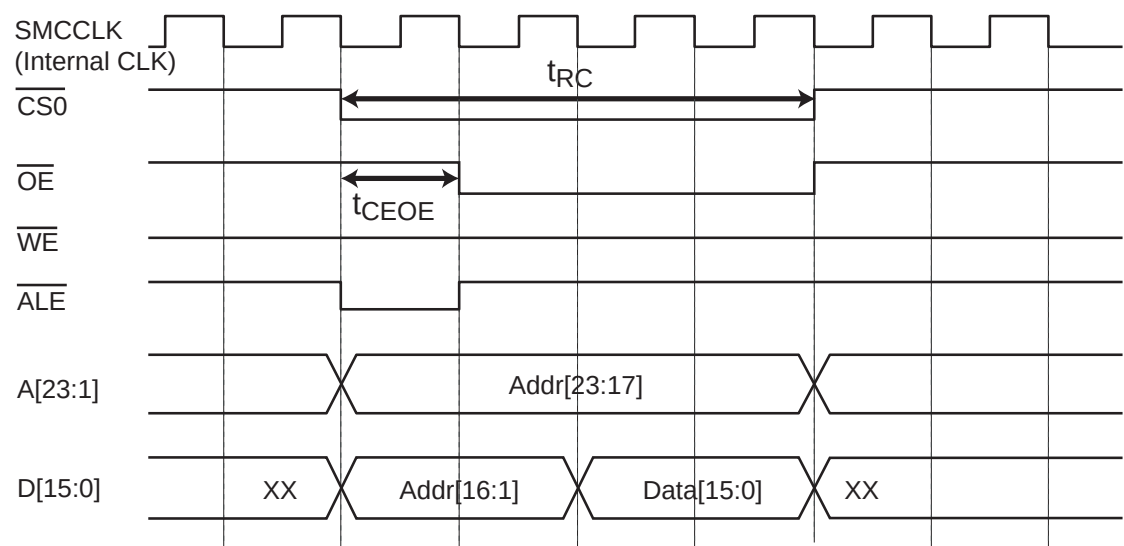
Figure 10-2 Asynchronous Read
