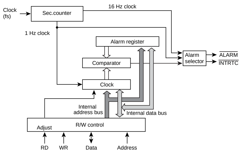
Figure 23-1 Block Diagram
