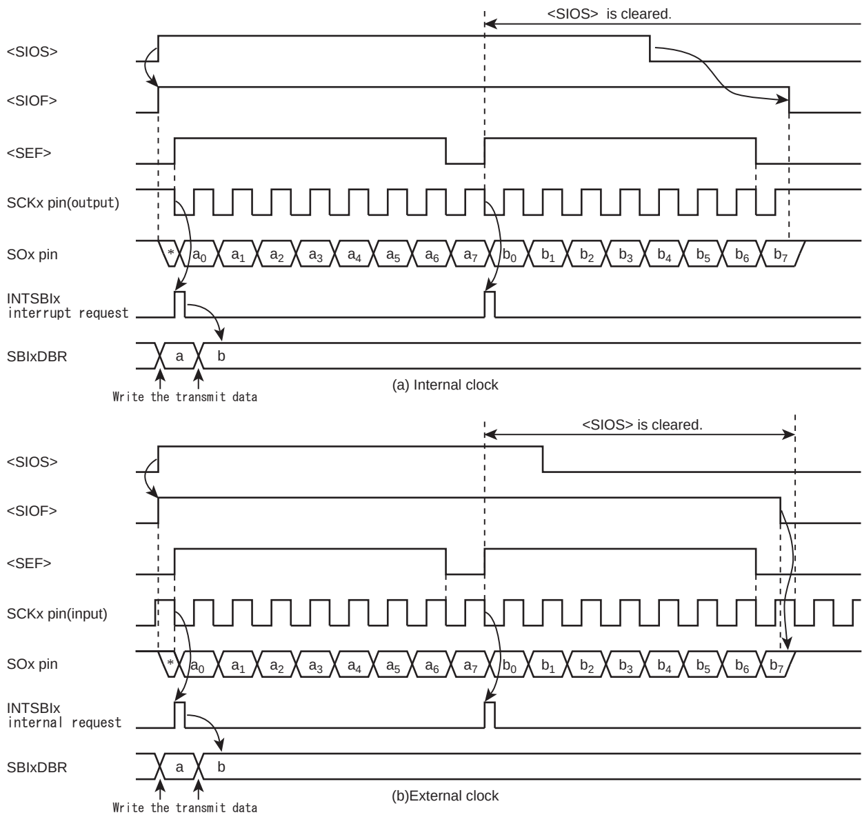
Figure 14-18 Transmit Mode
