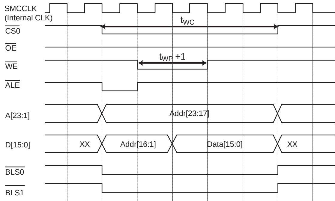
Figure 10-3 Asynchronous Write
