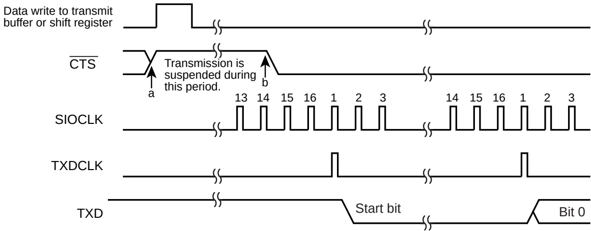
Figure 12-9 \overline{\text{CTS}} Signal timing
