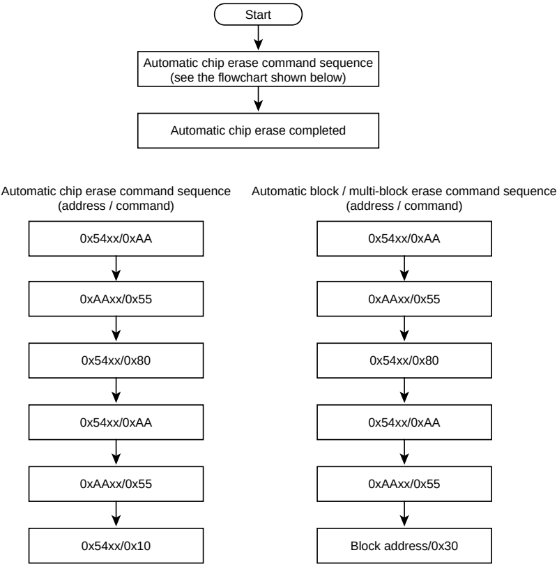
Figure 24-11 Automatic Erase
