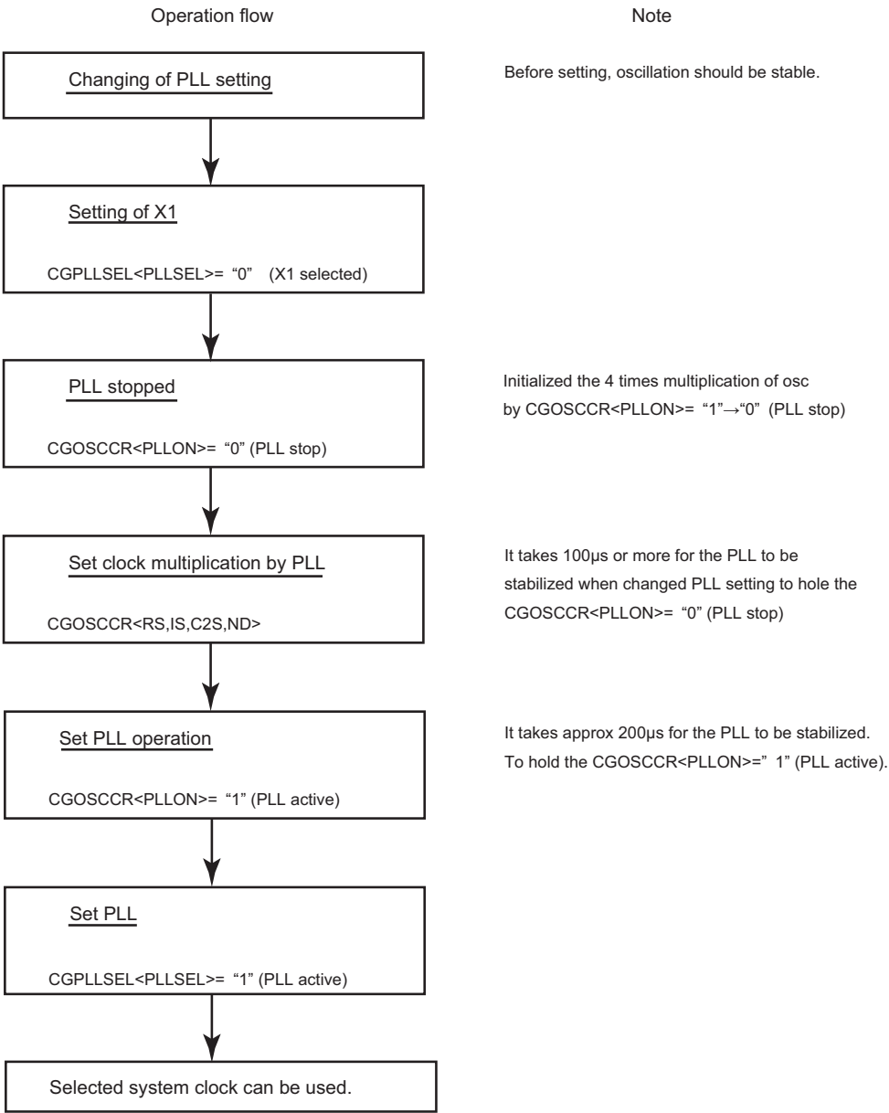
Figure 6-3 Changing the PLL setting
