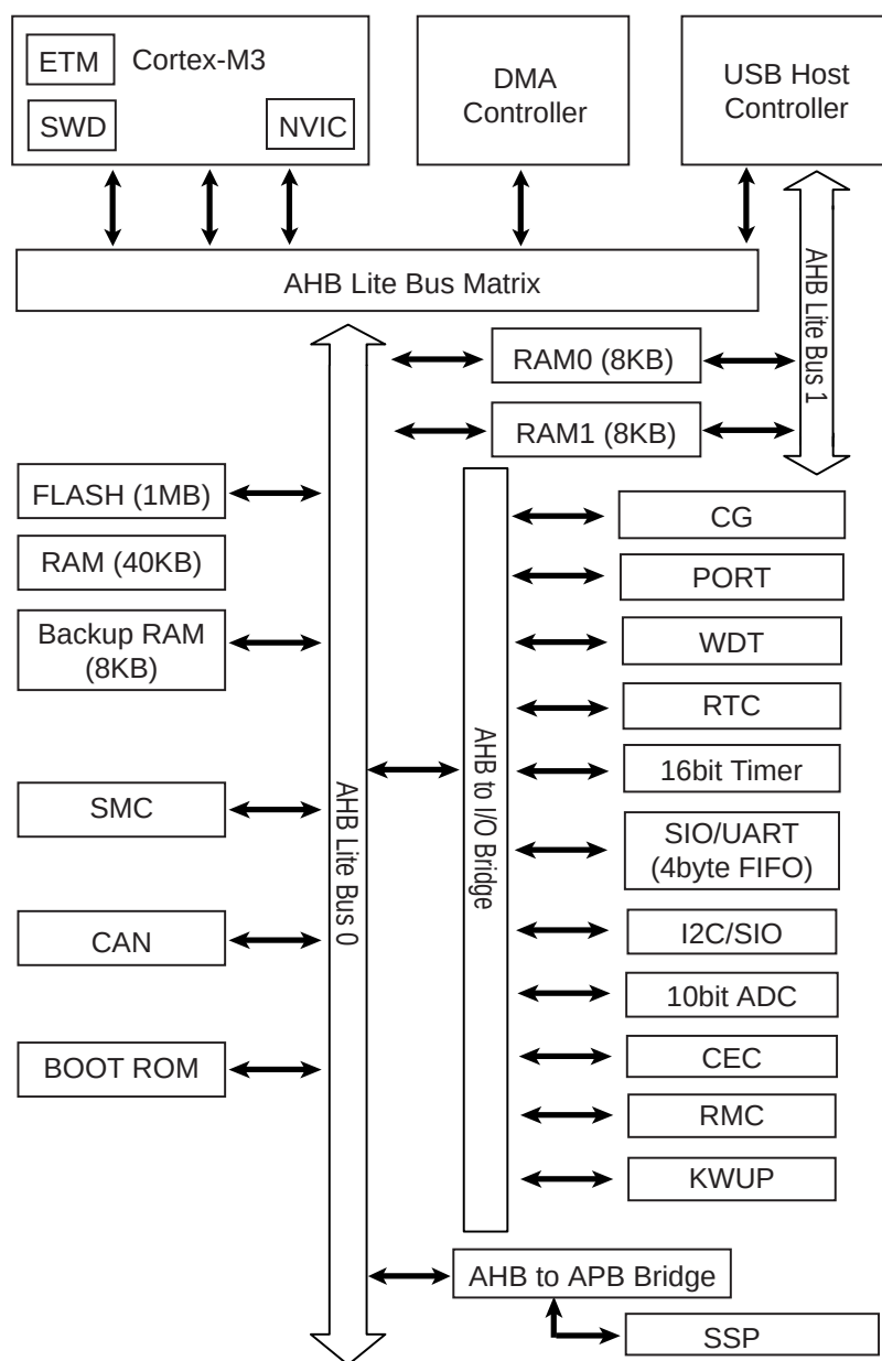
Figure 1-1 TMPM363F10FG Block Diagram
