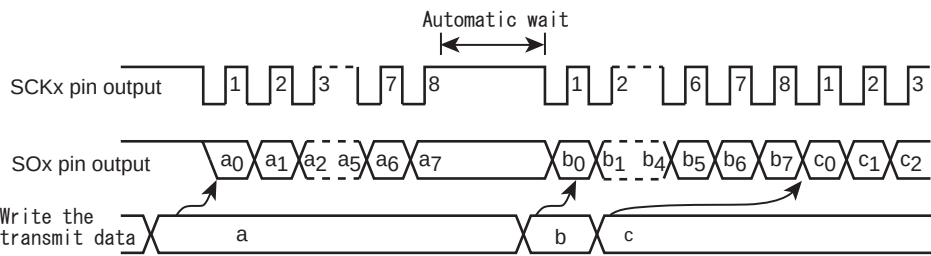
Figure 14-15 Automatic Wait
