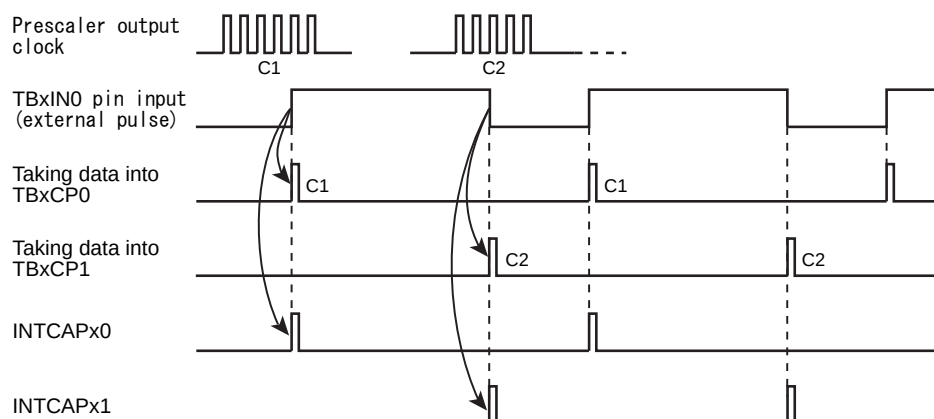
Figure 11-9 Pulse Width Measurement
