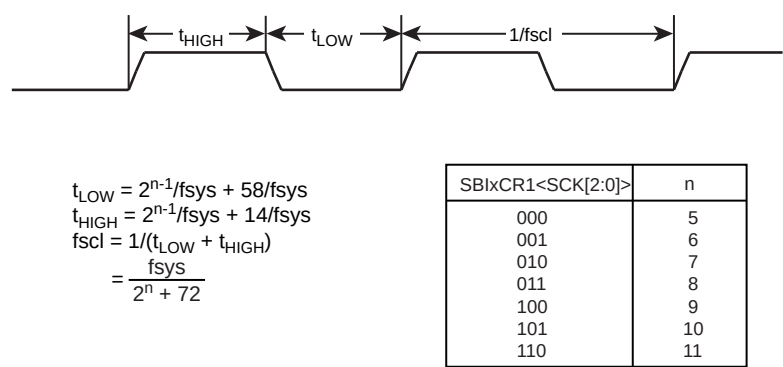
Figure 14-3 Clock source
