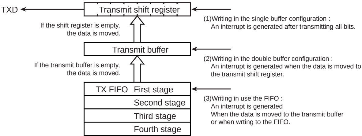
Figure 12-11 Transmit Buffer / FIFO Configuration Diagram
