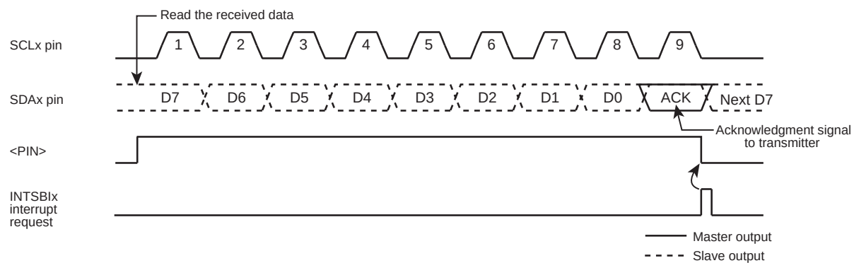
Figure 14-11 <BC[2:0]>= "000",<ACK>= "1" (Receiver Mode)
