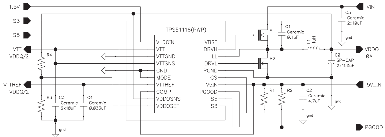
Figure 5. D-CAP™ Mode, PWP Package
