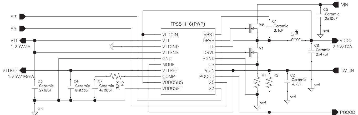
Figure 7. Current Mode, PWP Package
