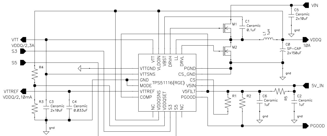
Figure 6. D-CAP™ Mode, RGE Package
