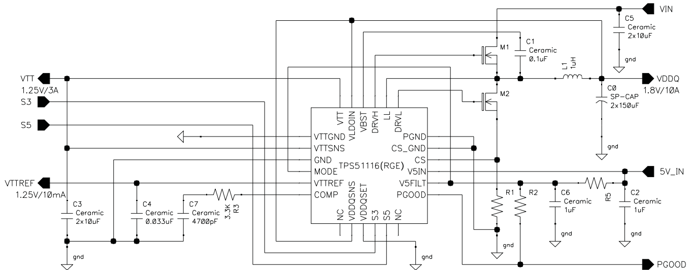
Figure 8. Current Mode, RGE Package
