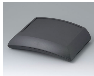
B7020209 ERGO-CASE L, flat ABS (UL 94 HB) black RAL 9005 5.91"x7.87"x2.13" IP 54 opt.
