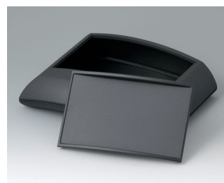
B7020139 ERGO-CASE L, flat ABS (UL 94 HB) black RAL 9005 5.91"x7.87"x2.13" IP 40
