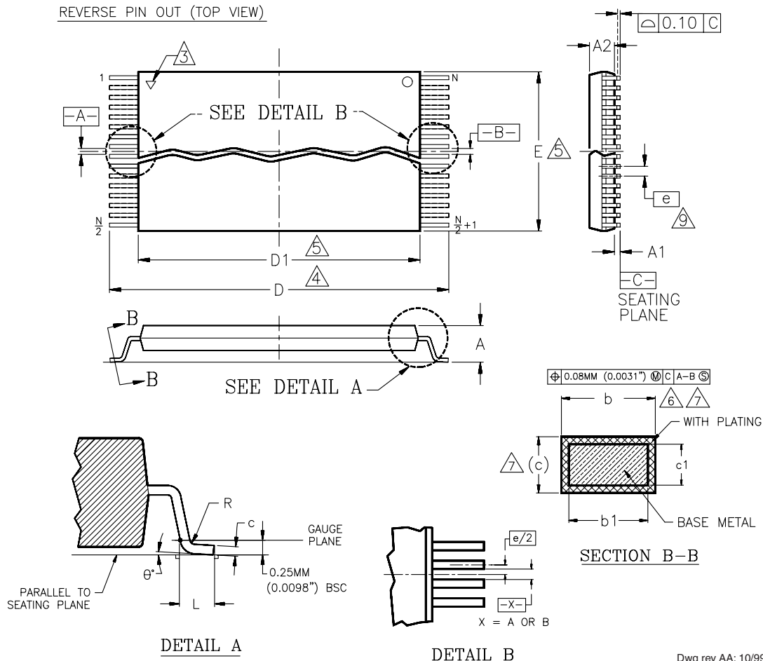
REVERSE PIN OUT (TOP VIEW)
