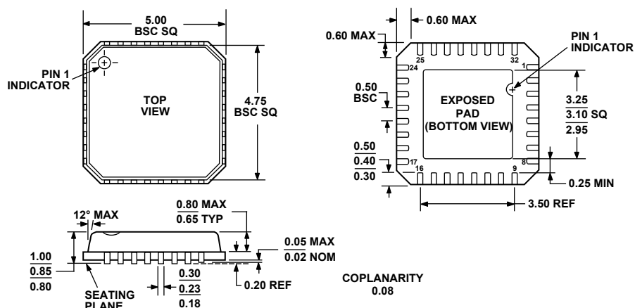
Figure 49. 32-Lead Lead Frame Chip Scale Package [LFCSP_VQ] 5 mm × 5 mm Body, Very Thin Quad (CP-32-2) Dimensions shown in millimeters
