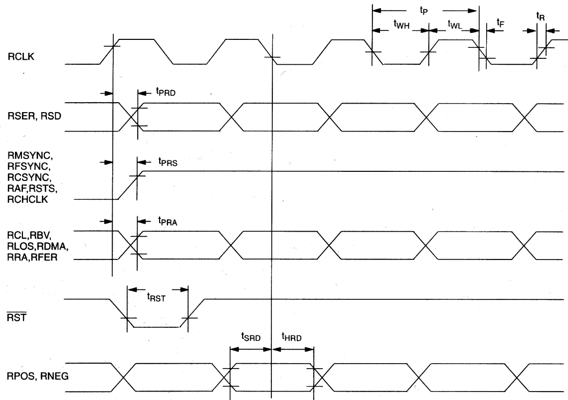
RECEIVE AC TIMING DIAGRAM Figure 31
