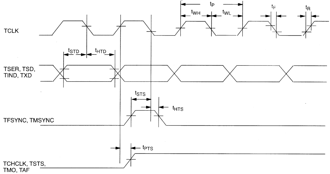
TRANSMIT AC TIMING DIAGRAM Figure 30
