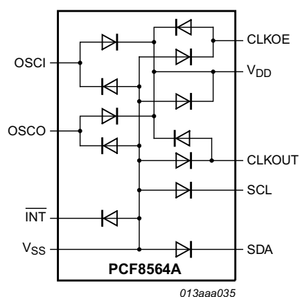
Fig 20. Device diode protection diagram
